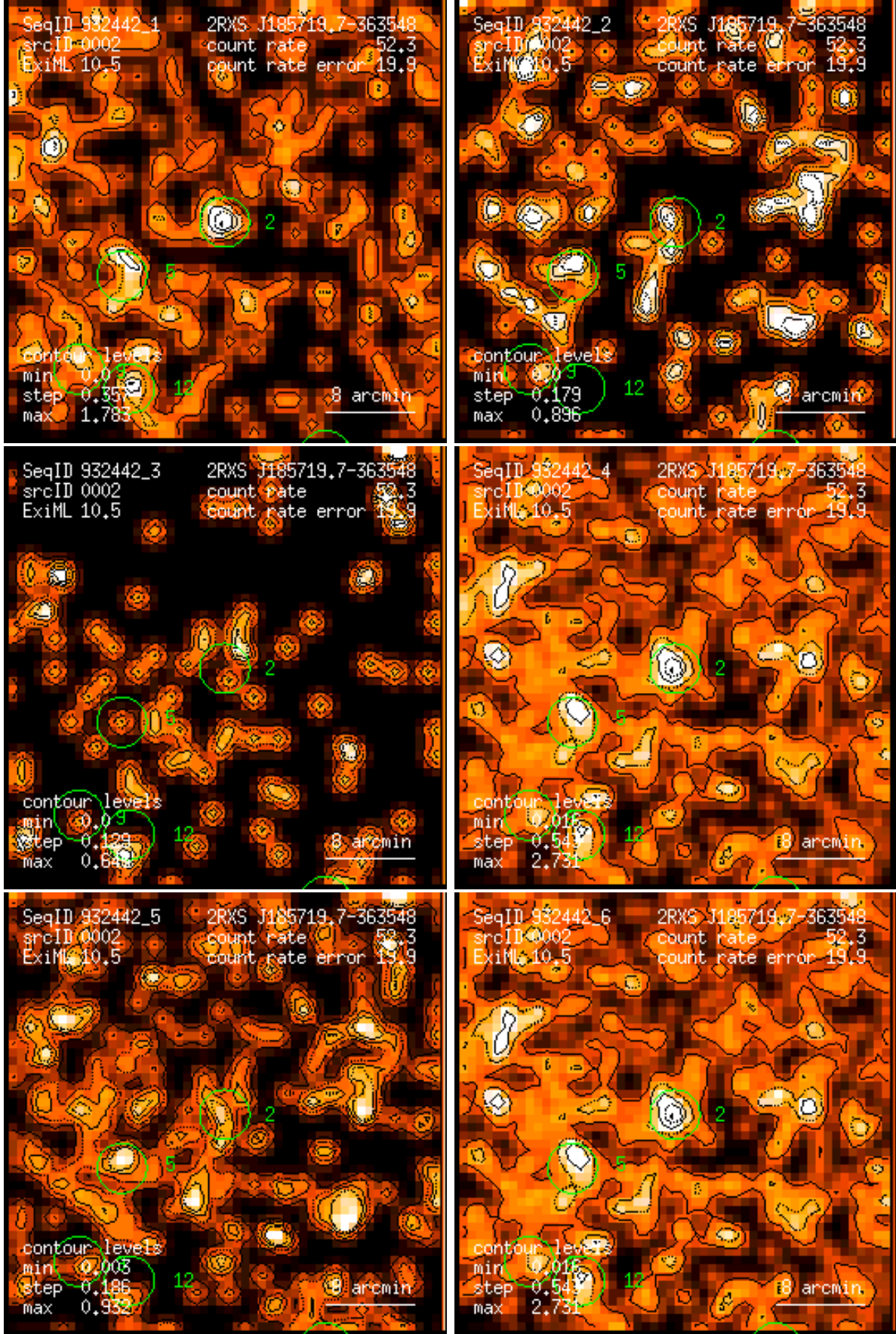
Figure 2: RASS 932442: detection 0002: band rate images, Gaussian filter: (1) PSPC channels 11 – 41, (2) 52 – 90, (3) 91 – 201, (4) 11 – 235, (5) 52 – 201, (6) 11 – 201. Broad band rates in counts/ks. Band rate contour levels in counts/ks/arcmin 2 .
