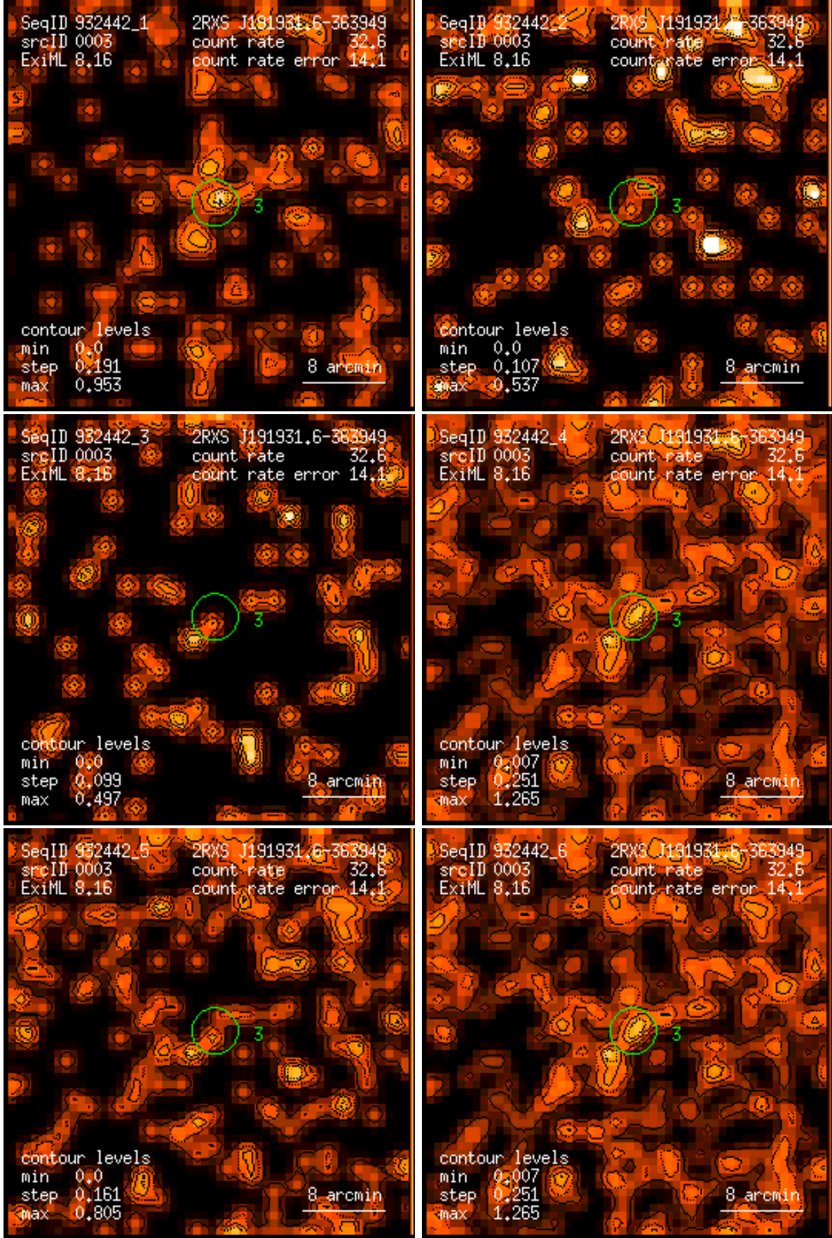
Figure 3: RASS 932442: detection 0003: band rate images, Gaussian filter: (1) PSPC channels 11 – 41, (2) 52 – 90, (3) 91 – 201, (4) 11 – 235, (5) 52 – 201, (6) 11 – 201. Broad band rates in counts/ks. Band rate contour levels in counts/ks/arcmin 2 .
