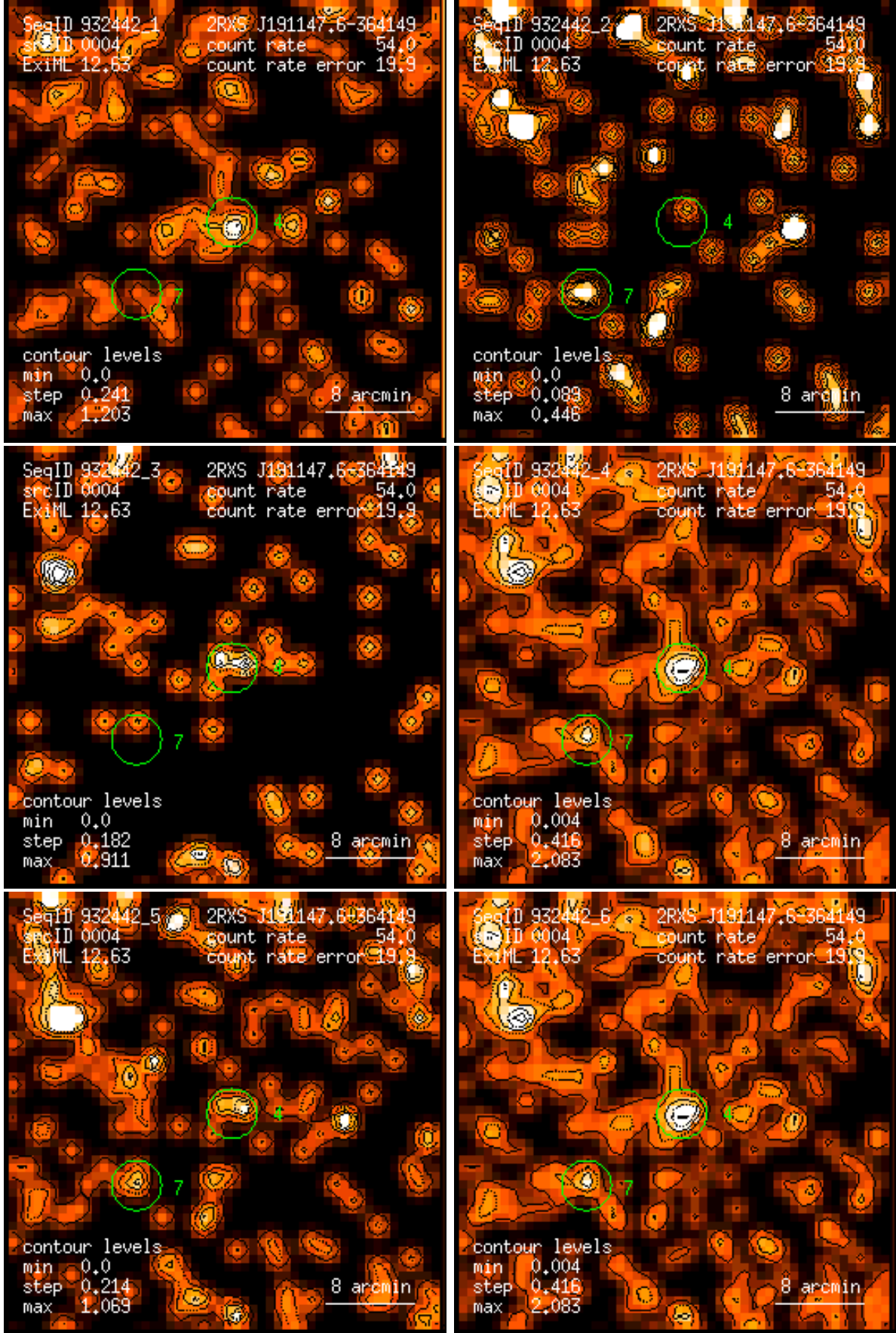
Figure 4: RASS 932442: detection 0004: band rate images, Gaussian filter: (1) PSPC channels 11 – 41, (2) 52 – 90, (3) 91 – 201, (4) 11 – 235, (5) 52 – 201, (6) 11 – 201. Broad band rates in counts/ks. Band rate contour levels in counts/ks/arcmin 2 .
