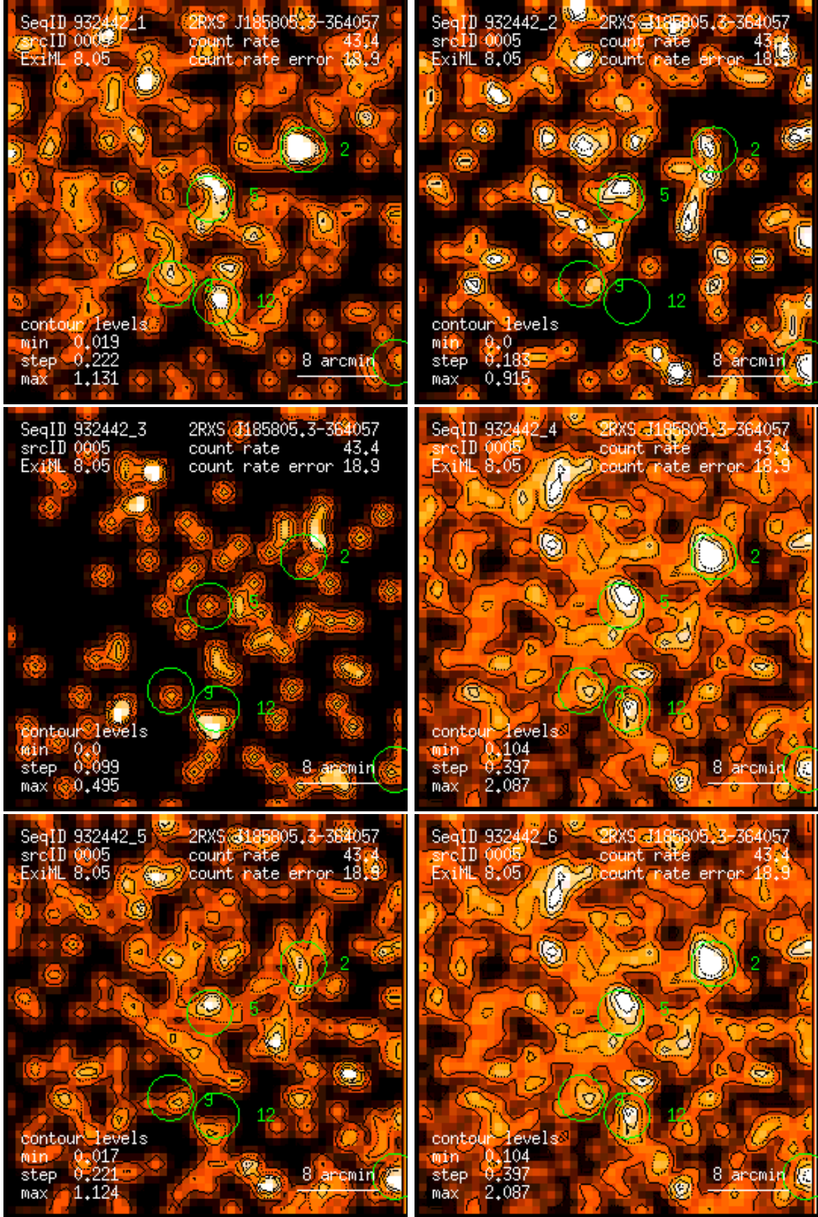
Figure 5: RASS 932442: detection 0005: band rate images, Gaussian filter: (1) PSPC channels 11 – 41, (2) 52 – 90, (3) 91 – 201, (4) 11 – 235, (5) 52 – 201, (6) 11 – 201. Broad band rates in counts/ks. Band rate contour levels in counts/ks/arcmin 2 .
