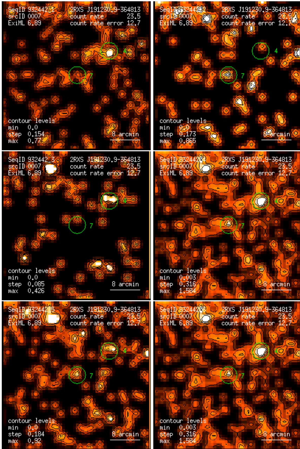
Figure 7: RASS 932442: detection 0007: band rate images, Gaussian filter: (1) PSPC channels 11 – 41, (2) 52 – 90, (3) 91 – 201, (4) 11 – 235, (5) 52 – 201, (6) 11 – 201. Broad band rates in counts/ks. Band rate contour levels in counts/ks/arcmin 2 .
