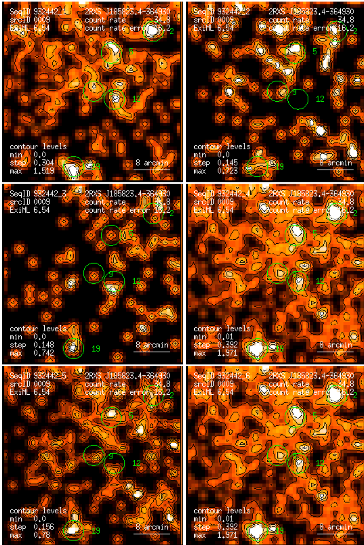
Figure 9: RASS 932442: detection 0009: band rate images, Gaussian filter: (1) PSPC channels 11 – 41, (2) 52 – 90, (3) 91 – 201, (4) 11 – 235, (5) 52 – 201, (6) 11 – 201. Broad band rates in counts/ks. Band rate contour levels in counts/ks/arcmin 2 .
