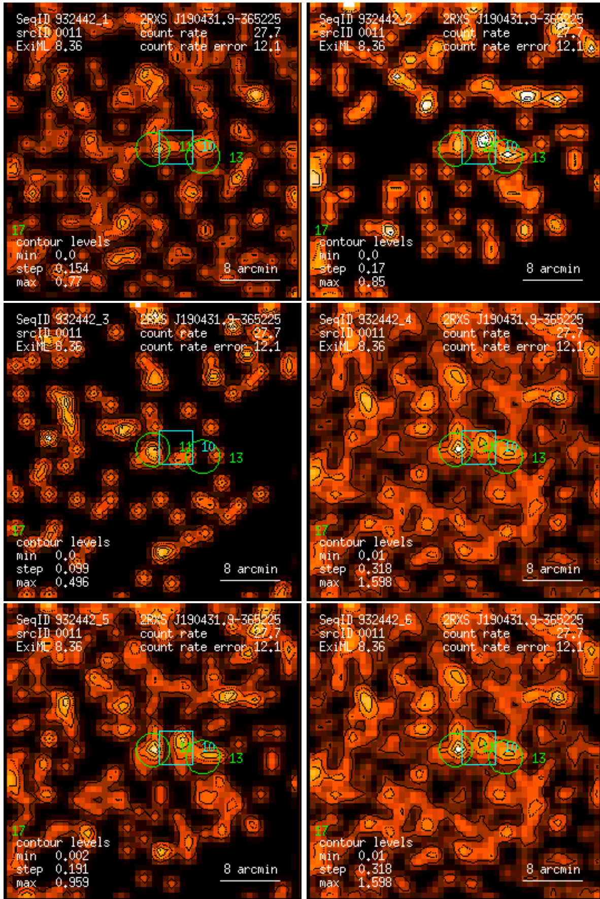
Figure 11: RASS 932442: detection 0011: band rate images, Gaussian filter: (1) PSPC channels 11 – 41, (2) 52 – 90, (3) 91 – 201, (4) 11 – 235, (5) 52 – 201, (6) 11 – 201. Broad band rates in counts/ks. Band rate contour levels in counts/ks/arcmin 2 .
