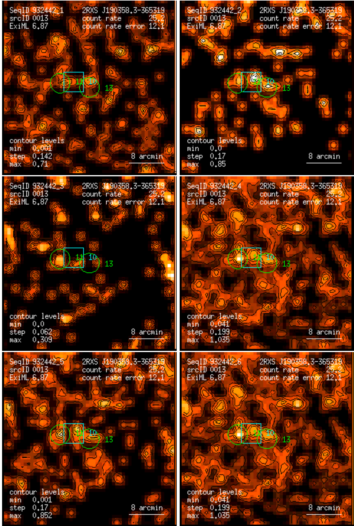
Figure 13: RASS 932442: detection 0013: band rate images, Gaussian filter: (1) PSPC channels 11 – 41, (2) 52 – 90, (3) 91 – 201, (4) 11 – 235, (5) 52 – 201, (6) 11 – 201. Broad band rates in counts/ks. Band rate contour levels in counts/ks/arcmin 2 .
