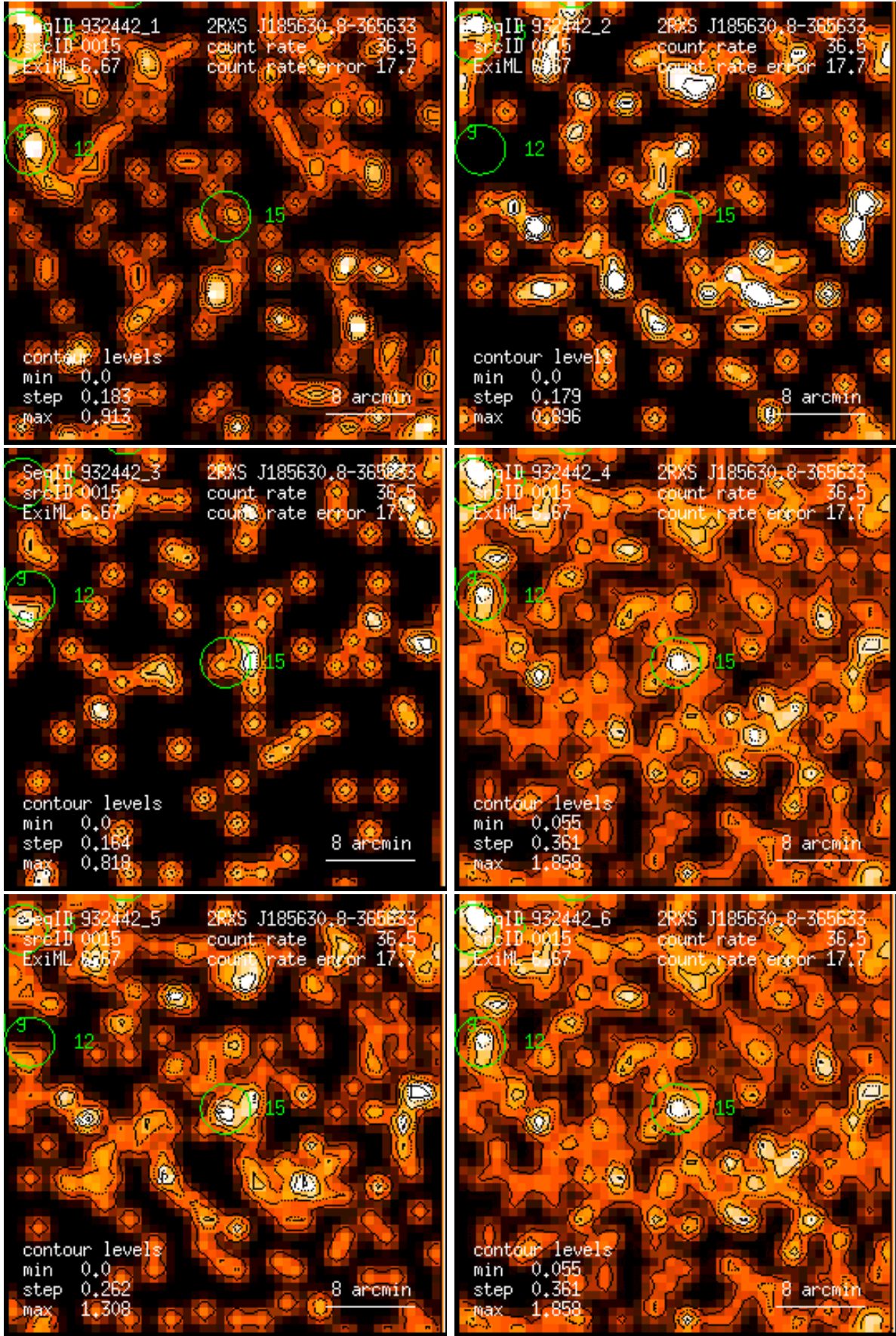
Figure 15: RASS 932442: detection 0015: band rate images, Gaussian filter: (1) PSPC channels 11 – 41, (2) 52 – 90, (3) 91 – 201, (4) 11 – 235, (5) 52 – 201, (6) 11 – 201. Broad band rates in counts/ks. Band rate contour levels in counts/ks/arcmin 2 .
