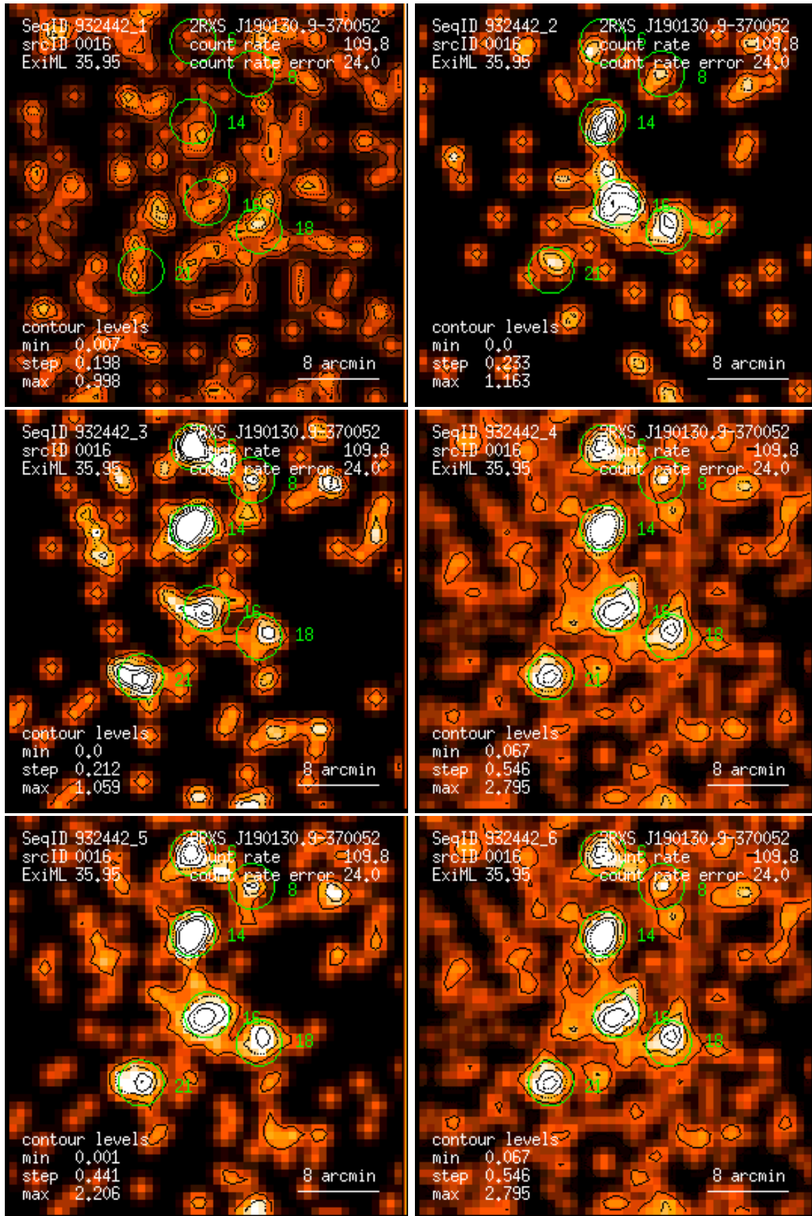
Figure 16: RASS 932442: detection 0016: band rate images, Gaussian filter: (1) PSPC channels 11 – 41, (2) 52 – 90, (3) 91 – 201, (4) 11 – 235, (5) 52 – 201, (6) 11 – 201. Broad band rates in counts/ks. Band rate contour levels in counts/ks/arcmin 2 .
