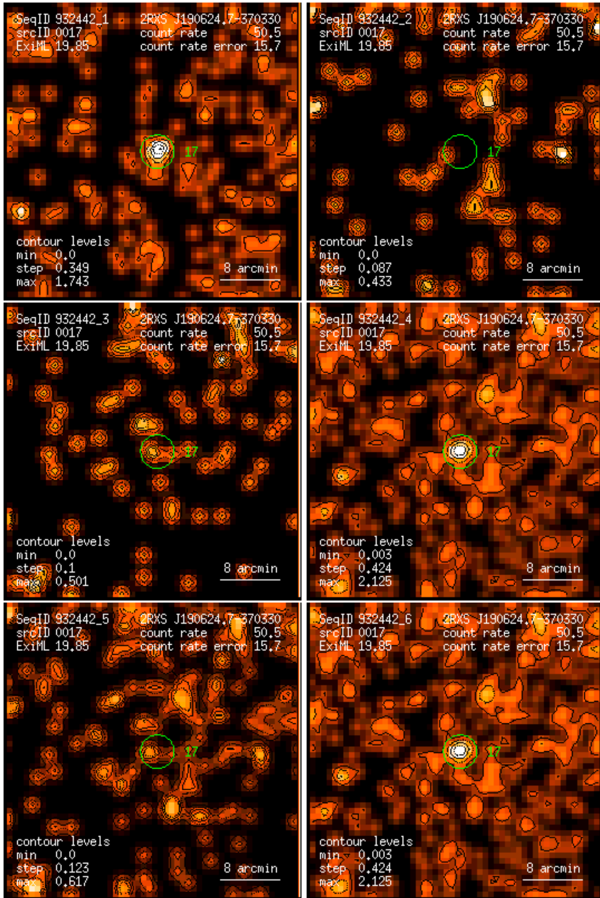
Figure 17: RASS 932442: detection 0017: band rate images, Gaussian filter: (1) PSPC channels 11 – 41, (2) 52 – 90, (3) 91 – 201, (4) 11 – 235, (5) 52 – 201, (6) 11 – 201. Broad band rates in counts/ks. Band rate contour levels in counts/ks/arcmin 2 .
