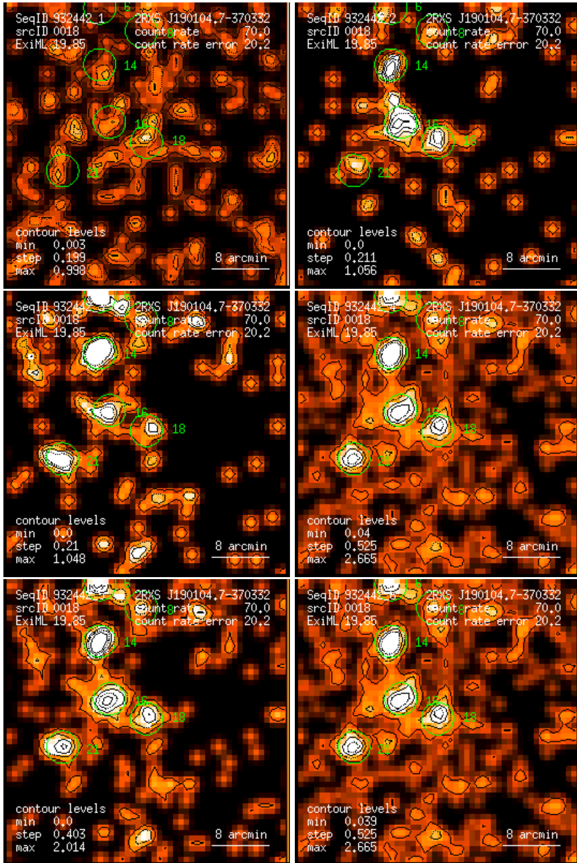
Figure 18: RASS 932442: detection 0018: band rate images, Gaussian filter: (1) PSPC channels 11 – 41, (2) 52 – 90, (3) 91 – 201, (4) 11 – 235, (5) 52 – 201, (6) 11 – 201. Broad band rates in counts/ks. Band rate contour levels in counts/ks/arcmin 2 .
