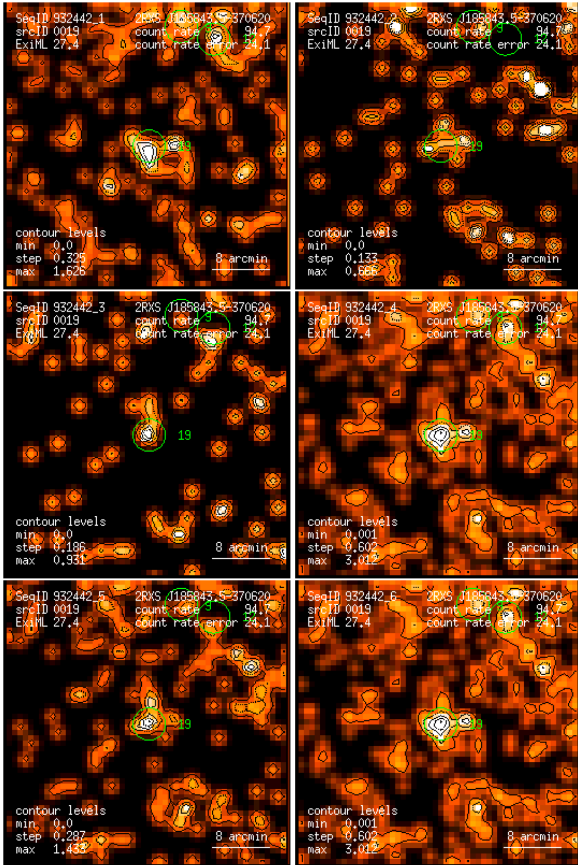
Figure 19: RASS 932442: detection 0019: band rate images, Gaussian filter: (1) PSPC channels 11 – 41, (2) 52 – 90, (3) 91 – 201, (4) 11 – 235, (5) 52 – 201, (6) 11 – 201. Broad band rates in counts/ks. Band rate contour levels in counts/ks/arcmin 2 .
