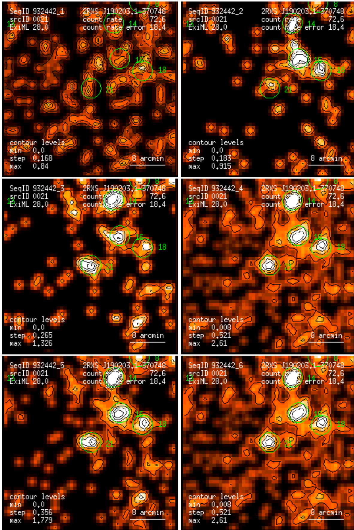
Figure 21: RASS 932442: detection 0021: band rate images, Gaussian filter: (1) PSPC channels 11 – 41, (2) 52 – 90, (3) 91 – 201, (4) 11 – 235, (5) 52 – 201, (6) 11 – 201. Broad band rates in counts/ks. Band rate contour levels in counts/ks/arcmin 2 .
