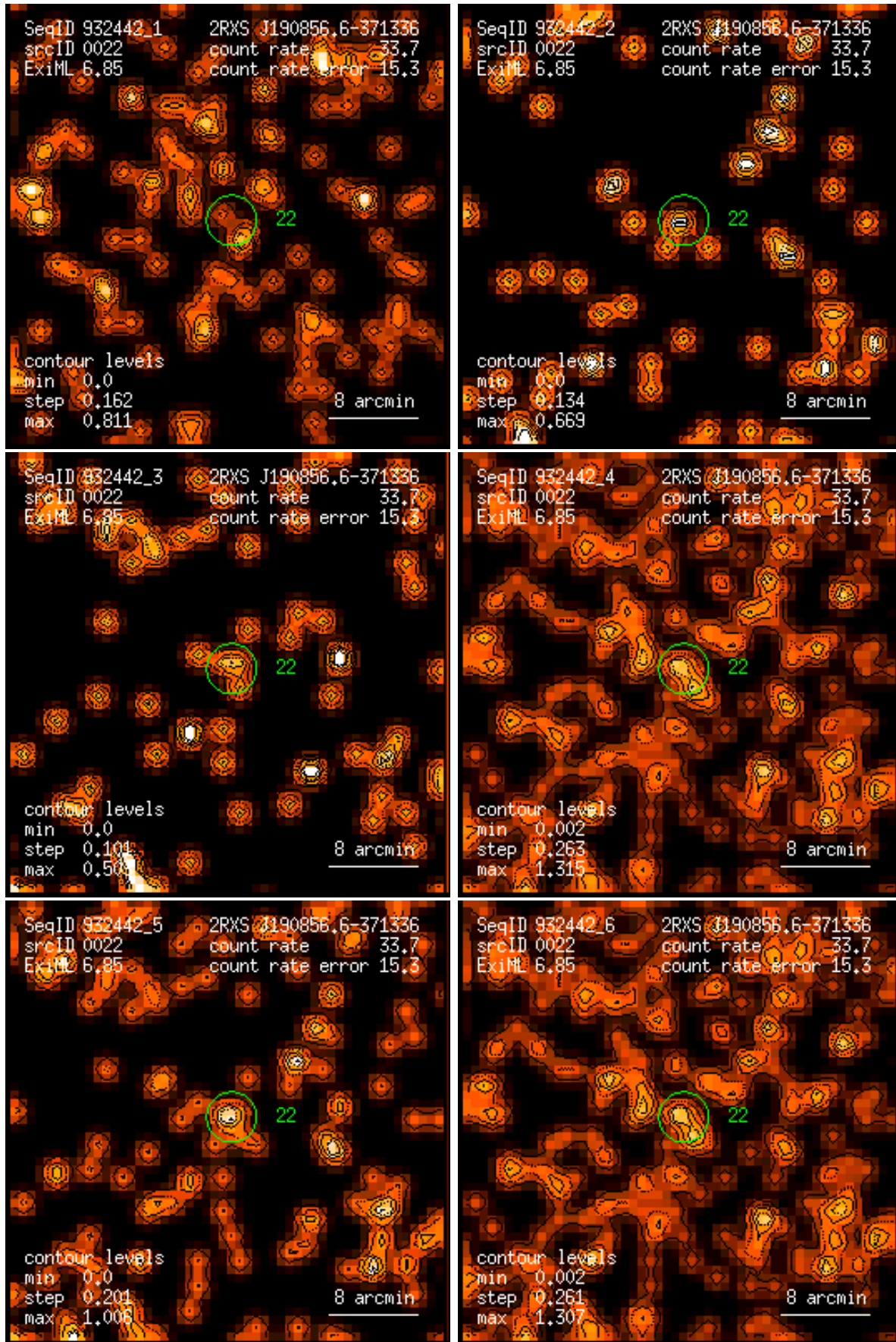
Figure 22: RASS 932442: detection 0022: band rate images, Gaussian filter: (1) PSPC channels 11 – 41, (2) 52 – 90, (3) 91 – 201, (4) 11 – 235, (5) 52 – 201, (6) 11 – 201. Broad band rates in counts/ks. Band rate contour levels in counts/ks/arcmin 2 .
