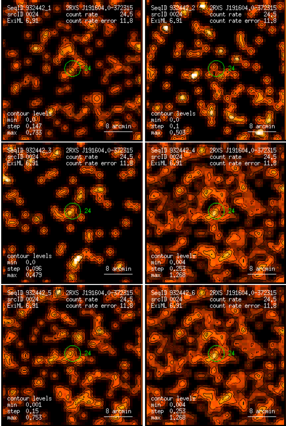
Figure 24: RASS 932442: detection 0024: band rate images, Gaussian filter: (1) PSPC channels 11 – 41, (2) 52 – 90, (3) 91 – 201, (4) 11 – 235, (5) 52 – 201, (6) 11 – 201. Broad band rates in counts/ks. Band rate contour levels in counts/ks/arcmin 2 .
