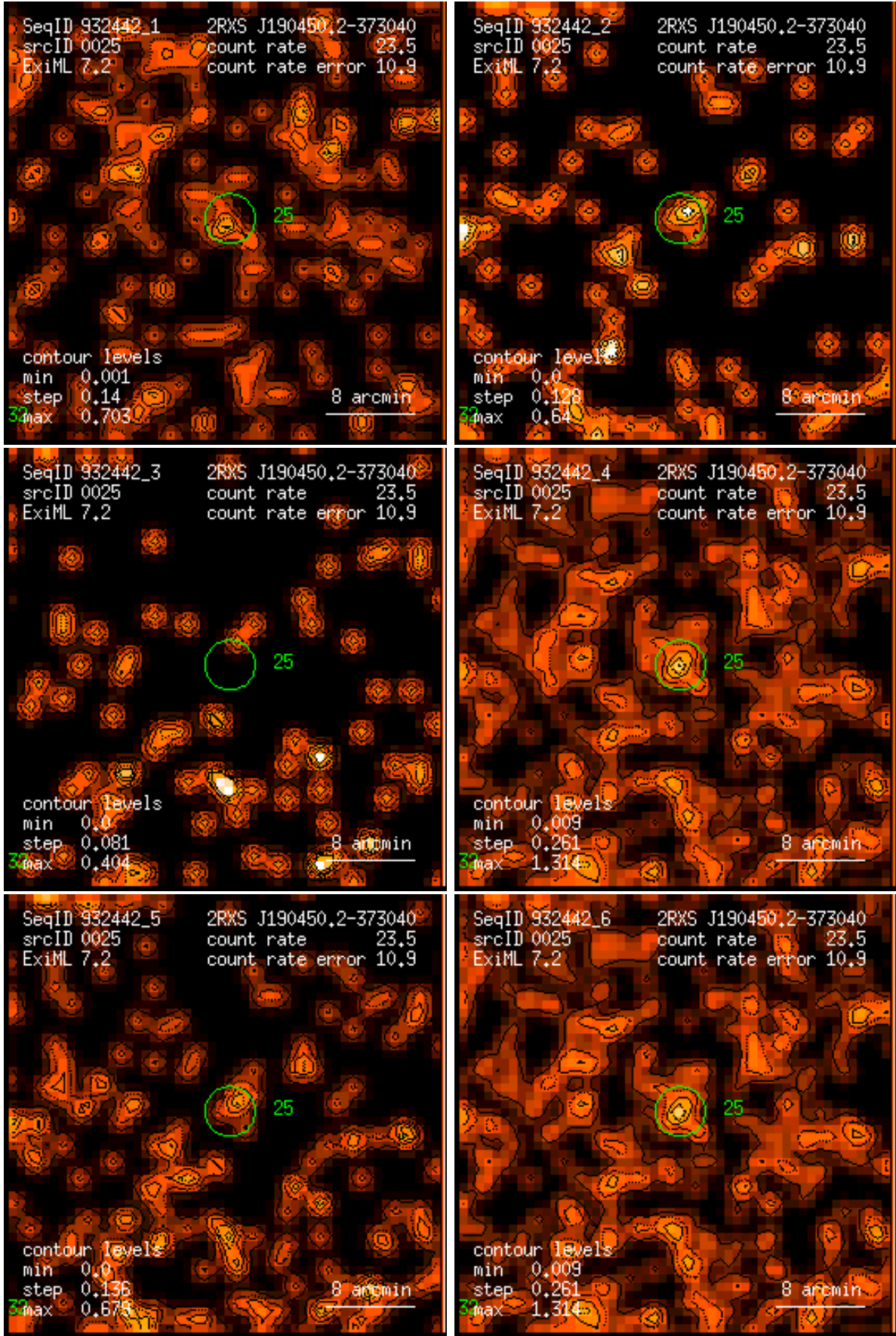
Figure 25: RASS 932442: detection 0025: band rate images, Gaussian filter: (1) PSPC channels 11 – 41, (2) 52 – 90, (3) 91 – 201, (4) 11 – 235, (5) 52 – 201, (6) 11 – 201. Broad band rates in counts/ks. Band rate contour levels in counts/ks/arcmin 2 .
