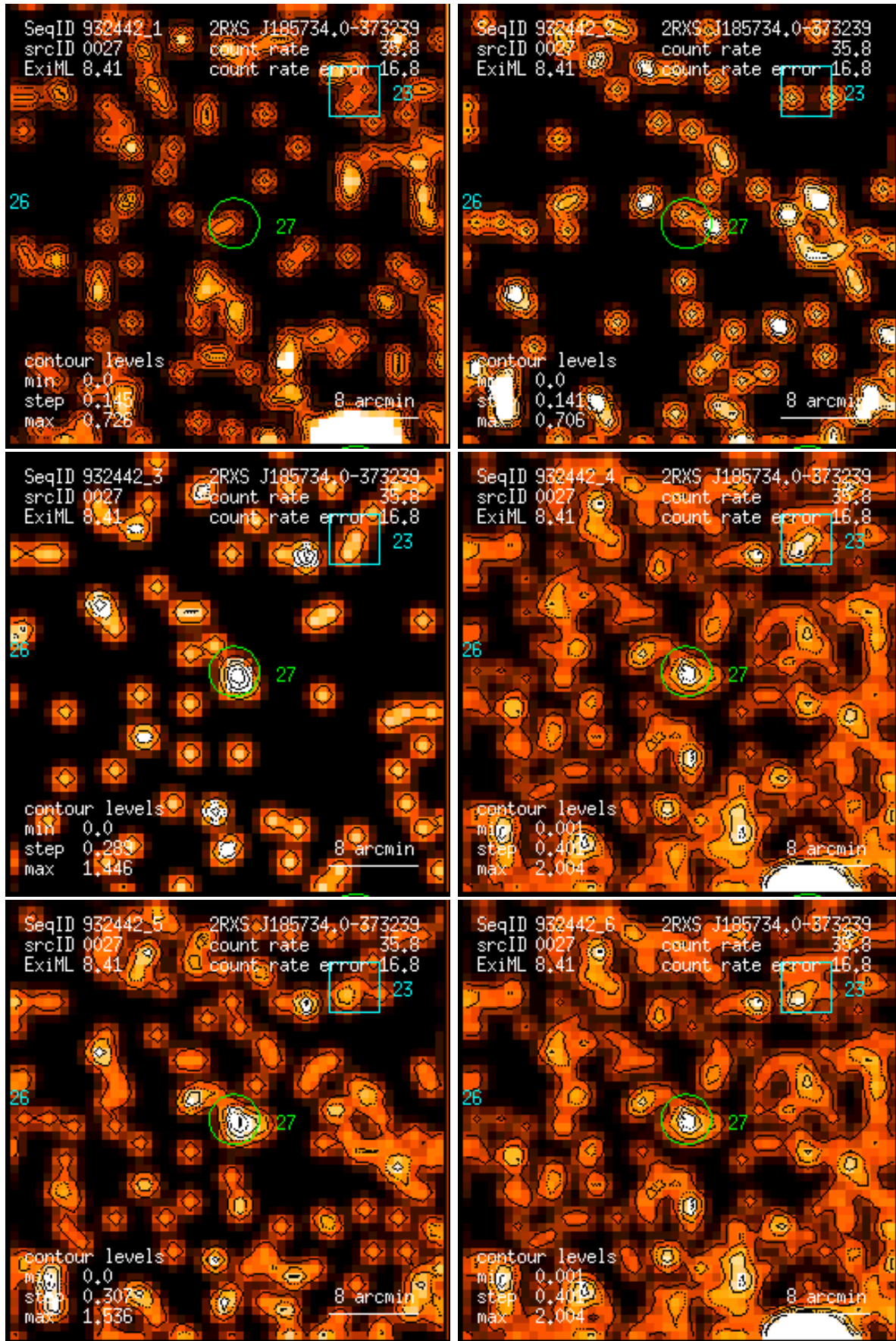
Figure 27: RASS 932442: detection 0027: band rate images, Gaussian filter: (1) PSPC channels 11 – 41, (2) 52 – 90, (3) 91 – 201, (4) 11 – 235, (5) 52 – 201, (6) 11 – 201. Broad band rates in counts/ks. Band rate contour levels in counts/ks/arcmin 2 .
