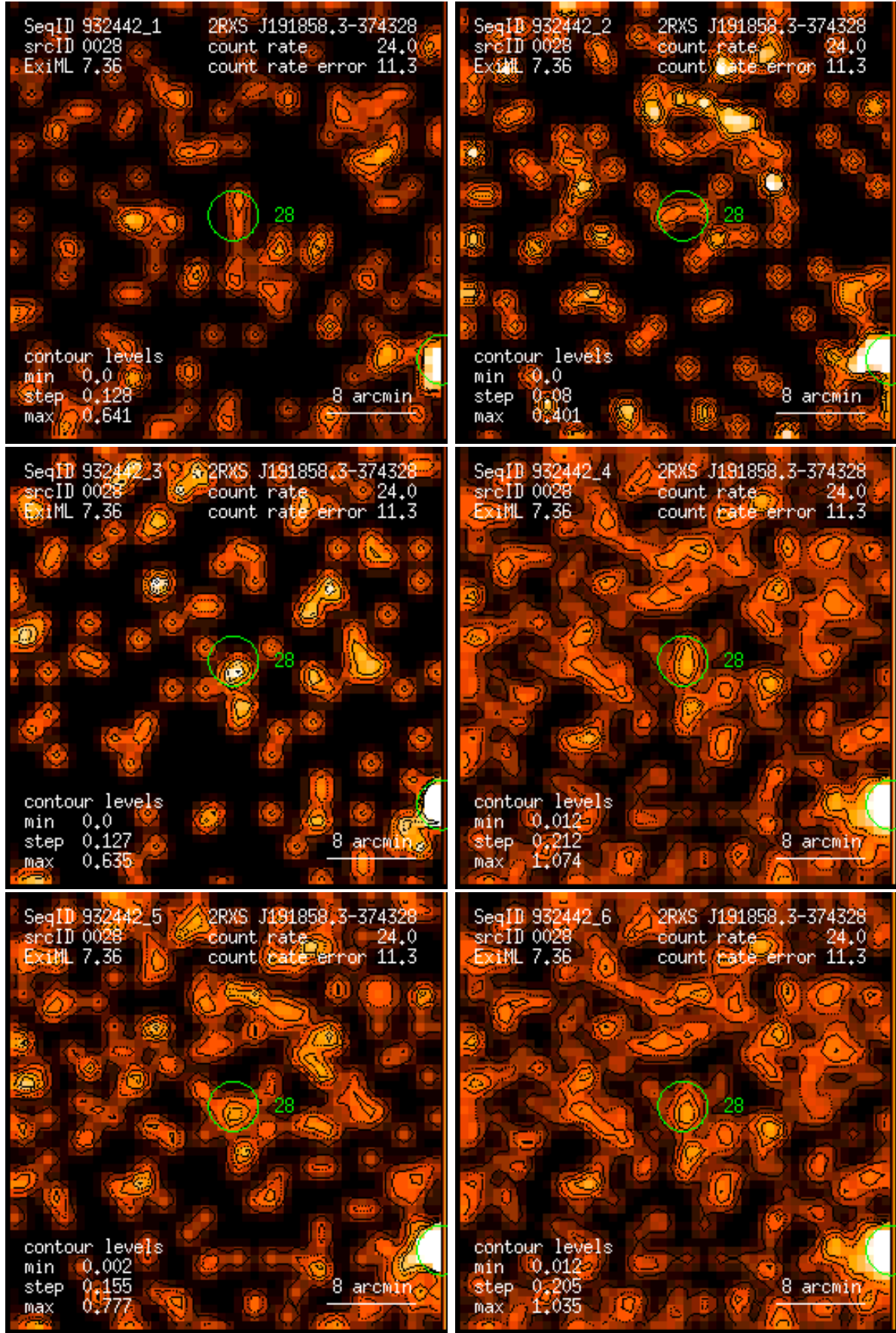
Figure 28: RASS 932442: detection 0028: band rate images, Gaussian filter: (1) PSPC channels 11 – 41, (2) 52 – 90, (3) 91 – 201, (4) 11 – 235, (5) 52 – 201, (6) 11 – 201. Broad band rates in counts/ks. Band rate contour levels in counts/ks/arcmin 2 .
