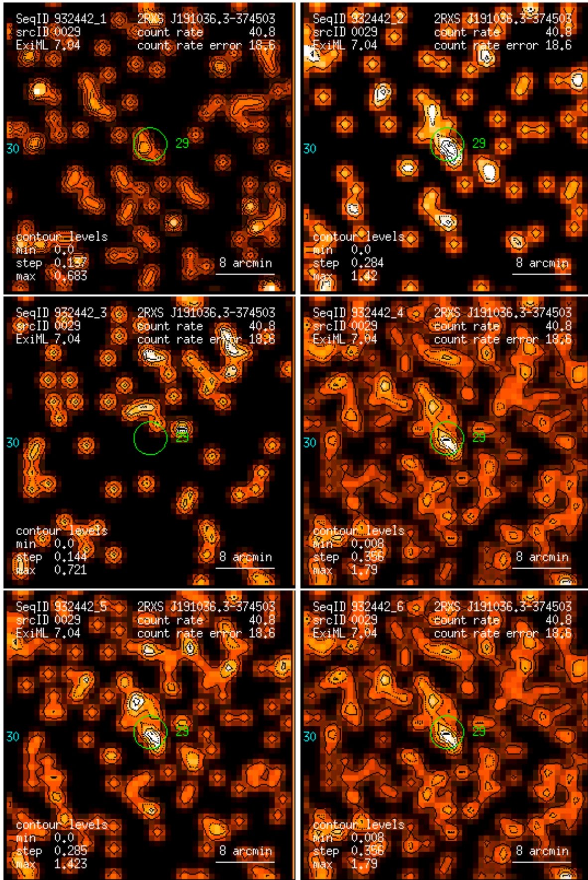
Figure 29: RASS 932442: detection 0029: band rate images, Gaussian filter: (1) PSPC channels 11 – 41, (2) 52 – 90, (3) 91 – 201, (4) 11 – 235, (5) 52 – 201, (6) 11 – 201. Broad band rates in counts/ks. Band rate contour levels in counts/ks/arcmin 2 .
