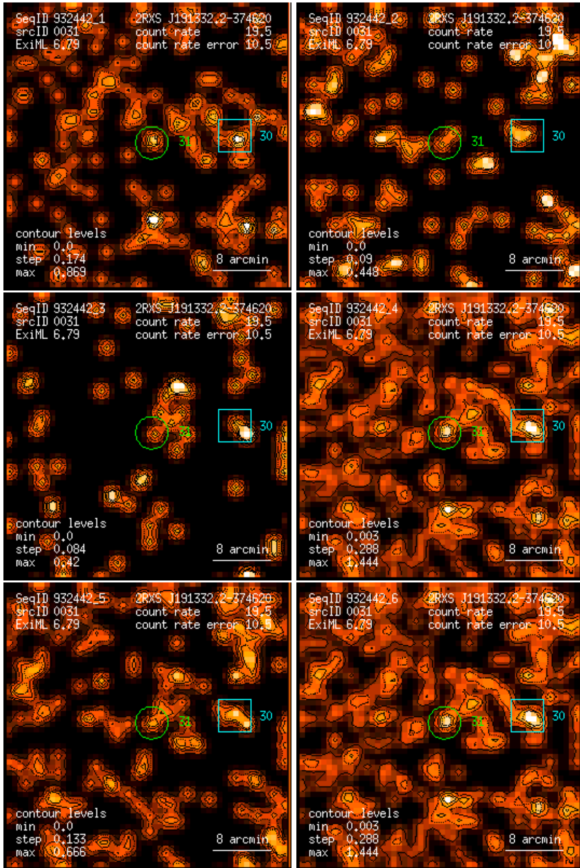
Figure 31: RASS 932442: detection 0031: band rate images, Gaussian filter: (1) PSPC channels 11 – 41, (2) 52 – 90, (3) 91 – 201, (4) 11 – 235, (5) 52 – 201, (6) 11 – 201. Broad band rates in counts/ks. Band rate contour levels in counts/ks/arcmin 2 .
