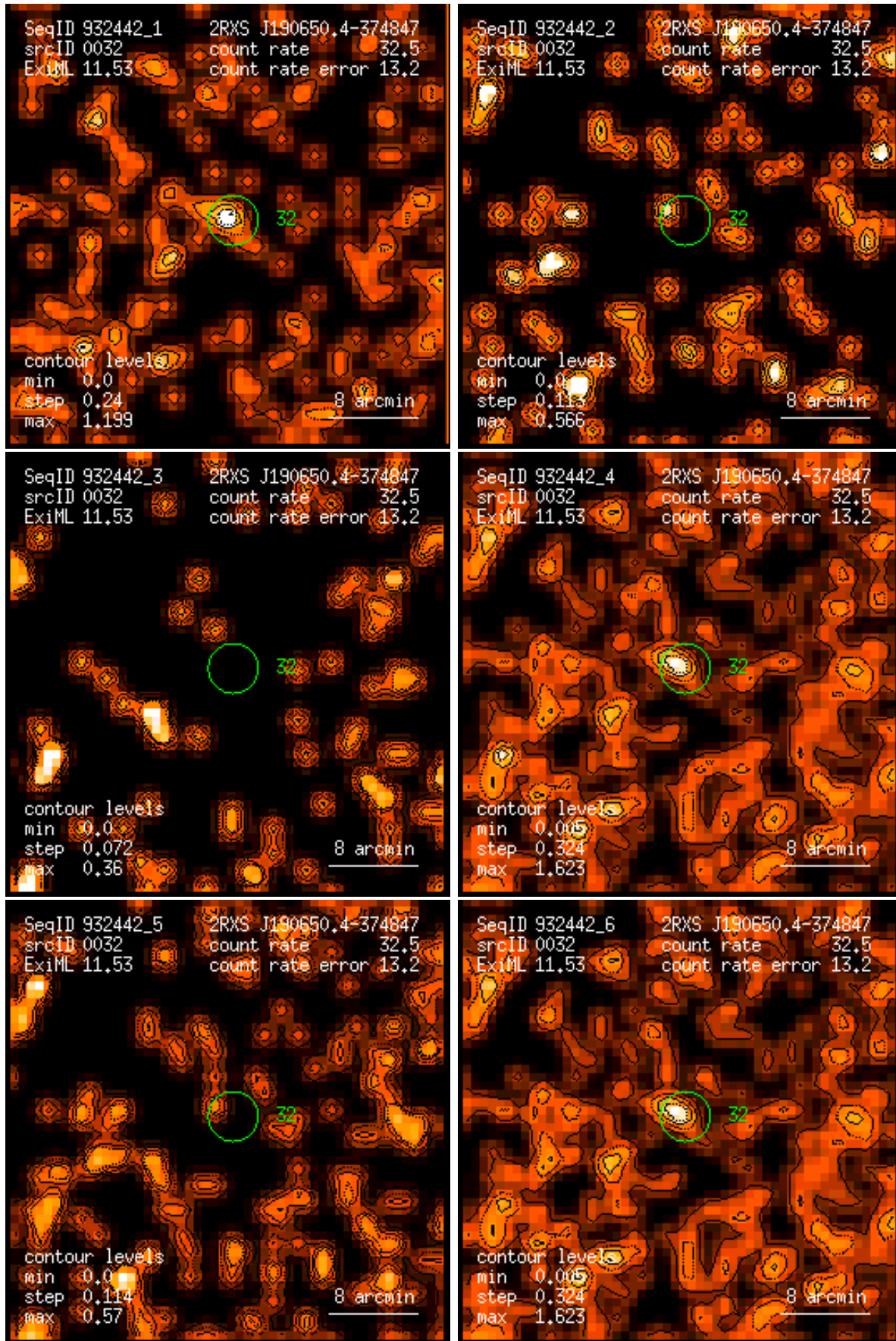
Figure 32: RASS 932442: detection 0032: band rate images, Gaussian filter: (1) PSPC channels 11 – 41, (2) 52 – 90, (3) 91 – 201, (4) 11 – 235, (5) 52 – 201, (6) 11 – 201. Broad band rates in counts/ks. Band rate contour levels in counts/ks/arcmin 2 .
