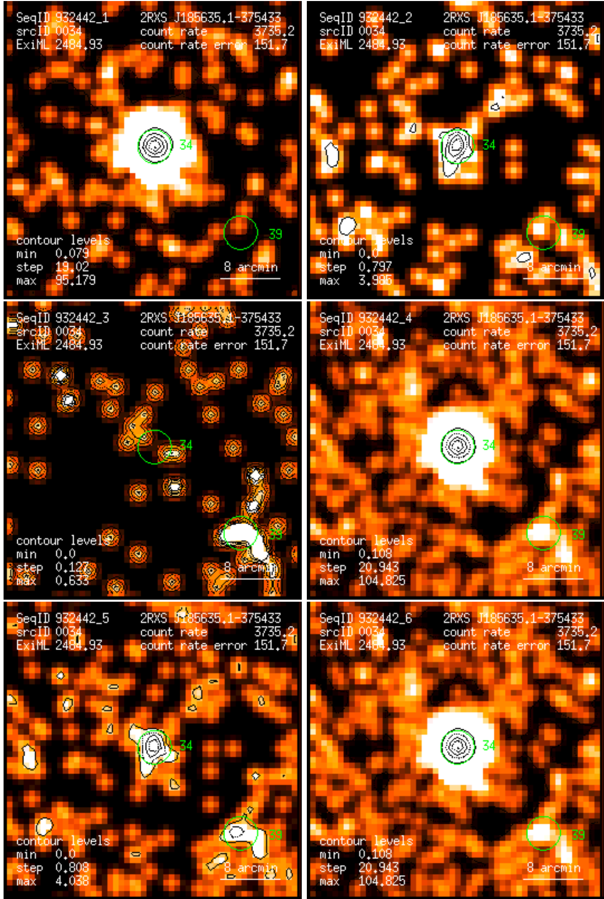
Figure 34: RASS 932442: detection 0034: band rate images, Gaussian filter: (1) PSPC channels 11 – 41, (2) 52 – 90, (3) 91 – 201, (4) 11 – 235, (5) 52 – 201, (6) 11 – 201. Broad band rates in counts/ks. Band rate contour levels in counts/ks/arcmin 2 .
