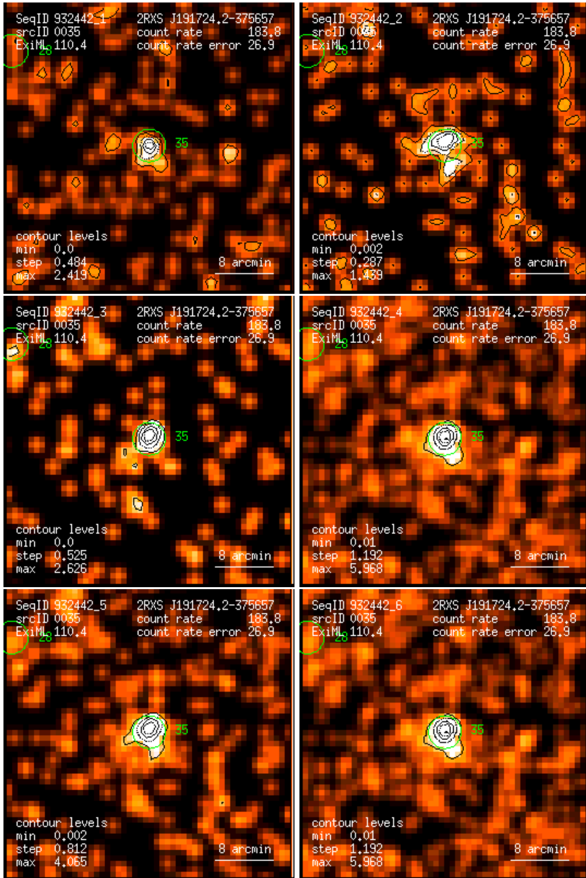
Figure 35: RASS 932442: detection 0035: band rate images, Gaussian filter: (1) PSPC channels 11 – 41, (2) 52 – 90, (3) 91 – 201, (4) 11 – 235, (5) 52 – 201, (6) 11 – 201. Broad band rates in counts/ks. Band rate contour levels in counts/ks/arcmin 2 .
