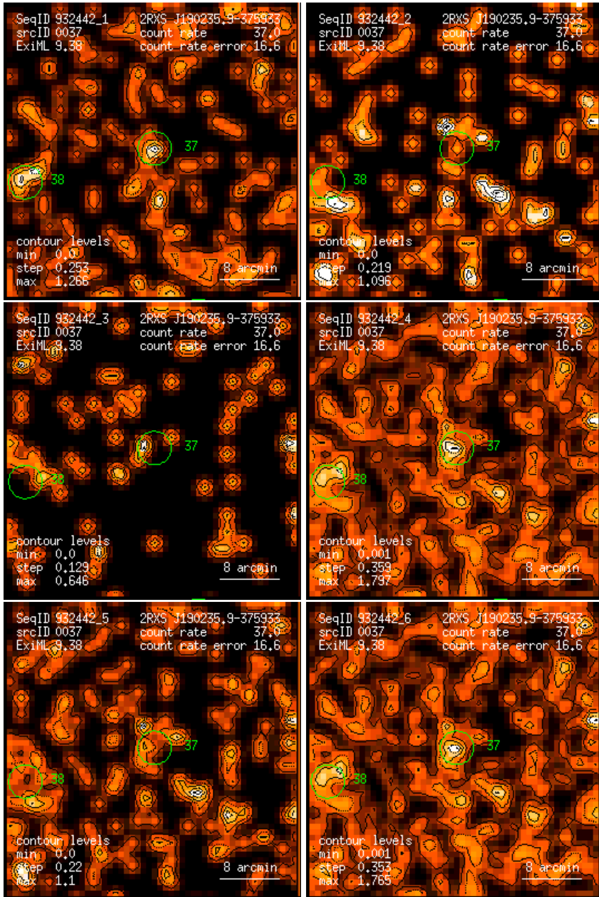
Figure 37: RASS 932442: detection 0037: band rate images, Gaussian filter: (1) PSPC channels 11 – 41, (2) 52 – 90, (3) 91 – 201, (4) 11 – 235, (5) 52 – 201, (6) 11 – 201. Broad band rates in counts/ks. Band rate contour levels in counts/ks/arcmin 2 .
