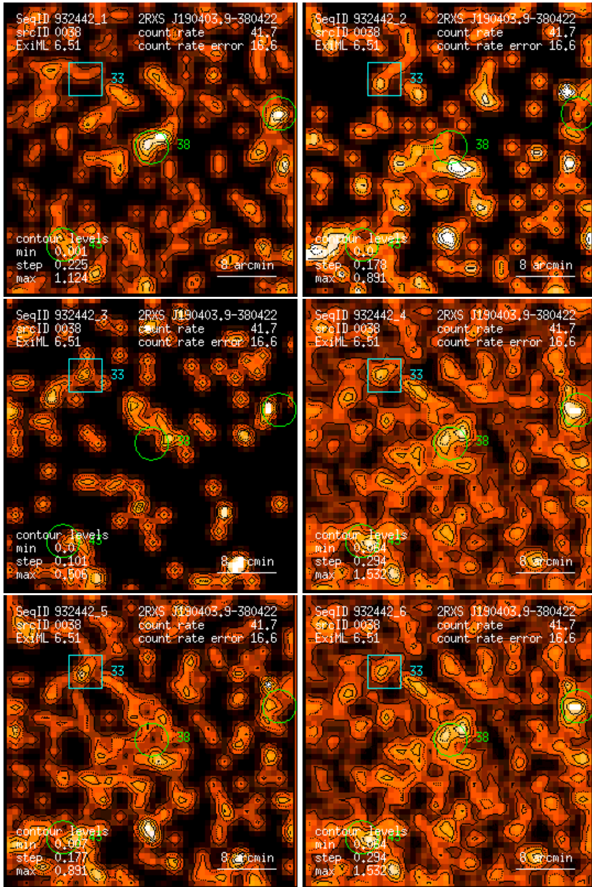
Figure 38: RASS 932442: detection 0038: band rate images, Gaussian filter: (1) PSPC channels 11 – 41, (2) 52 – 90, (3) 91 – 201, (4) 11 – 235, (5) 52 – 201, (6) 11 – 201. Broad band rates in counts/ks. Band rate contour levels in counts/ks/arcmin 2 .
