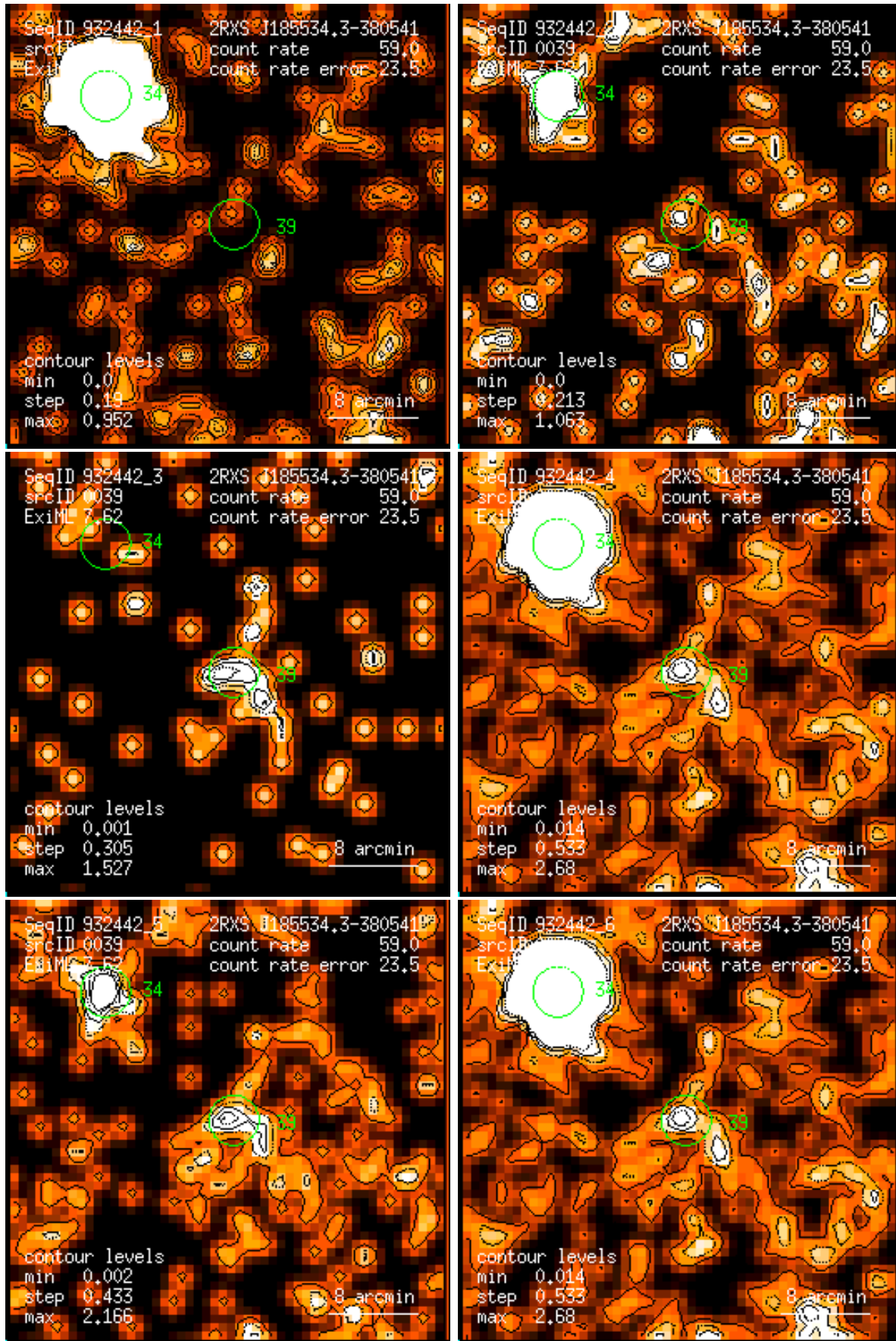
Figure 39: RASS 932442: detection 0039: band rate images, Gaussian filter: (1) PSPC channels 11 – 41, (2) 52 – 90, (3) 91 – 201, (4) 11 – 235, (5) 52 – 201, (6) 11 – 201. Broad band rates in counts/ks. Band rate contour levels in counts/ks/arcmin 2 .
