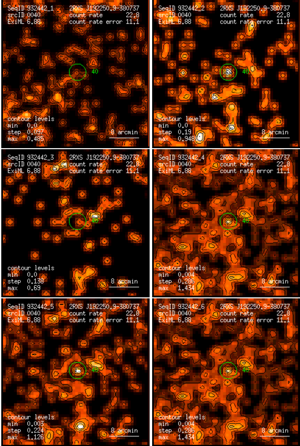
Figure 40: RASS 932442: detection 0040: band rate images, Gaussian filter: (1) PSPC channels 11 – 41, (2) 52 – 90, (3) 91 – 201, (4) 11 – 235, (5) 52 – 201, (6) 11 – 201. Broad band rates in counts/ks. Band rate contour levels in counts/ks/arcmin 2 .
