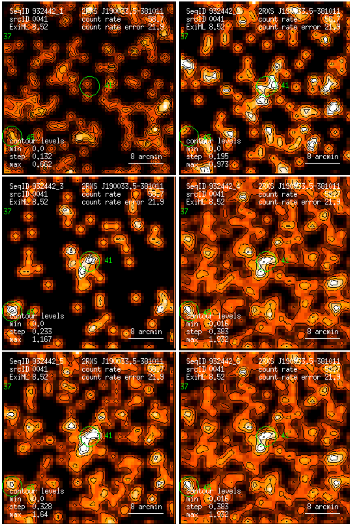
Figure 41: RASS 932442: detection 0041: band rate images, Gaussian filter: (1) PSPC channels 11 – 41, (2) 52 – 90, (3) 91 – 201, (4) 11 – 235, (5) 52 – 201, (6) 11 – 201. Broad band rates in counts/ks. Band rate contour levels in counts/ks/arcmin 2 .
