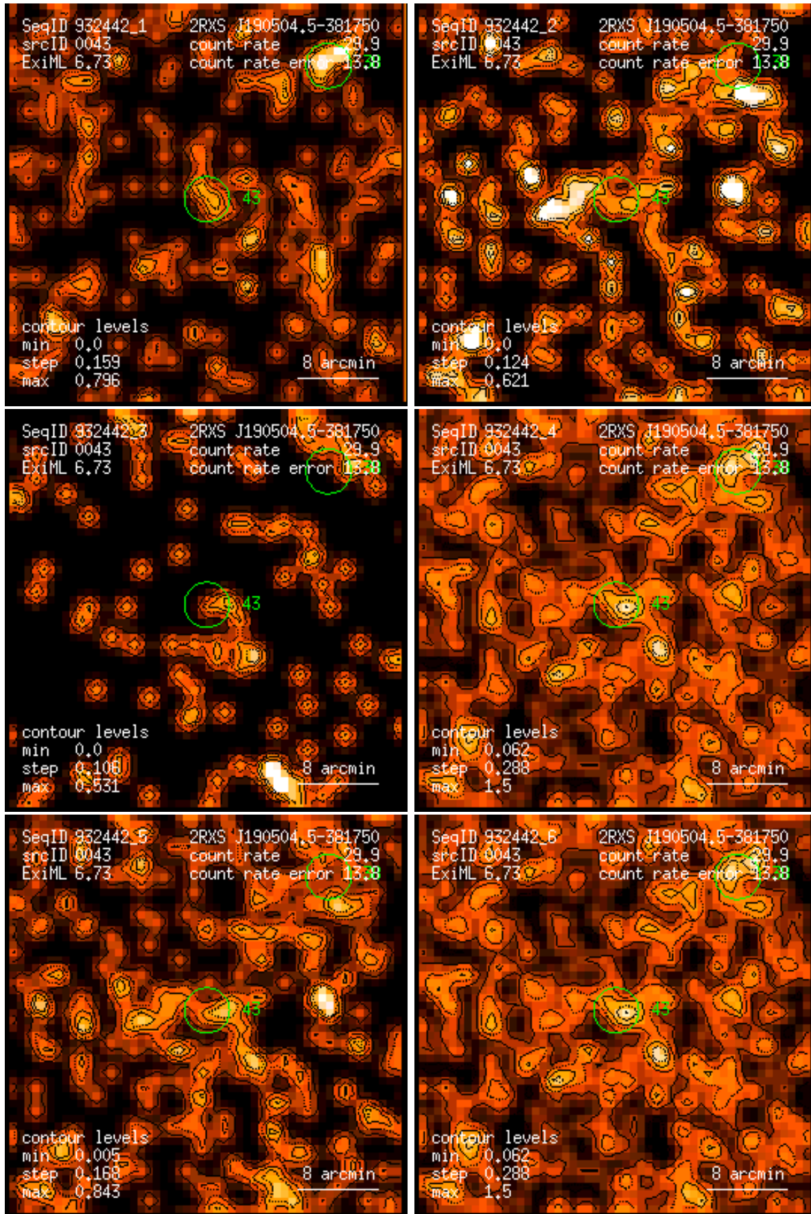
Figure 43: RASS 932442: detection 0043: band rate images, Gaussian filter: (1) PSPC channels 11 – 41, (2) 52 – 90, (3) 91 – 201, (4) 11 – 235, (5) 52 – 201, (6) 11 – 201. Broad band rates in counts/ks. Band rate contour levels in counts/ks/arcmin 2 .
