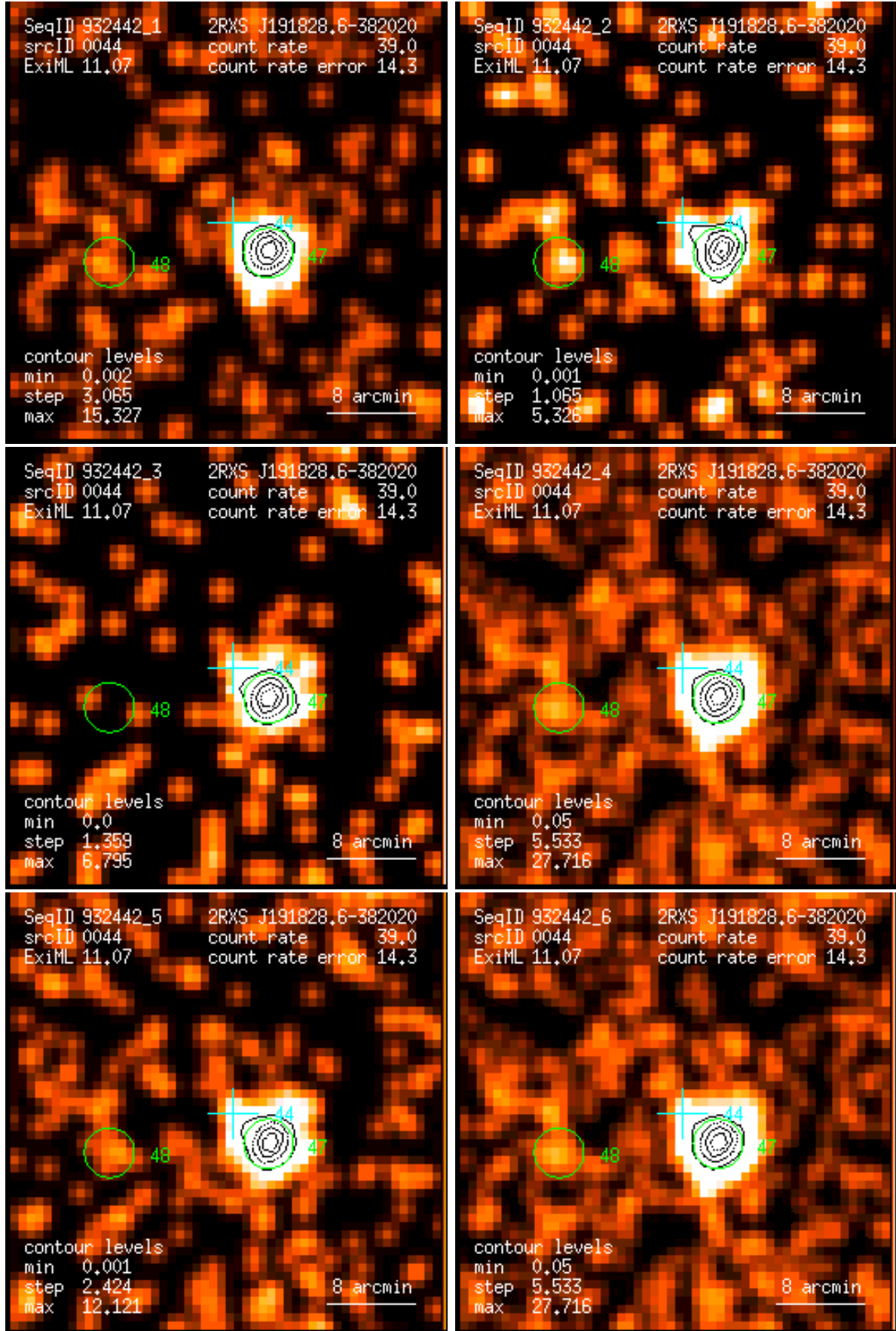
Figure 44: RASS 932442: detection 0044: band rate images, Gaussian filter: (1) PSPC channels 11 – 41, (2) 52 – 90, (3) 91 – 201, (4) 11 – 235, (5) 52 – 201, (6) 11 – 201. Broad band rates in counts/ks. Band rate contour levels in counts/ks/arcmin 2 .
