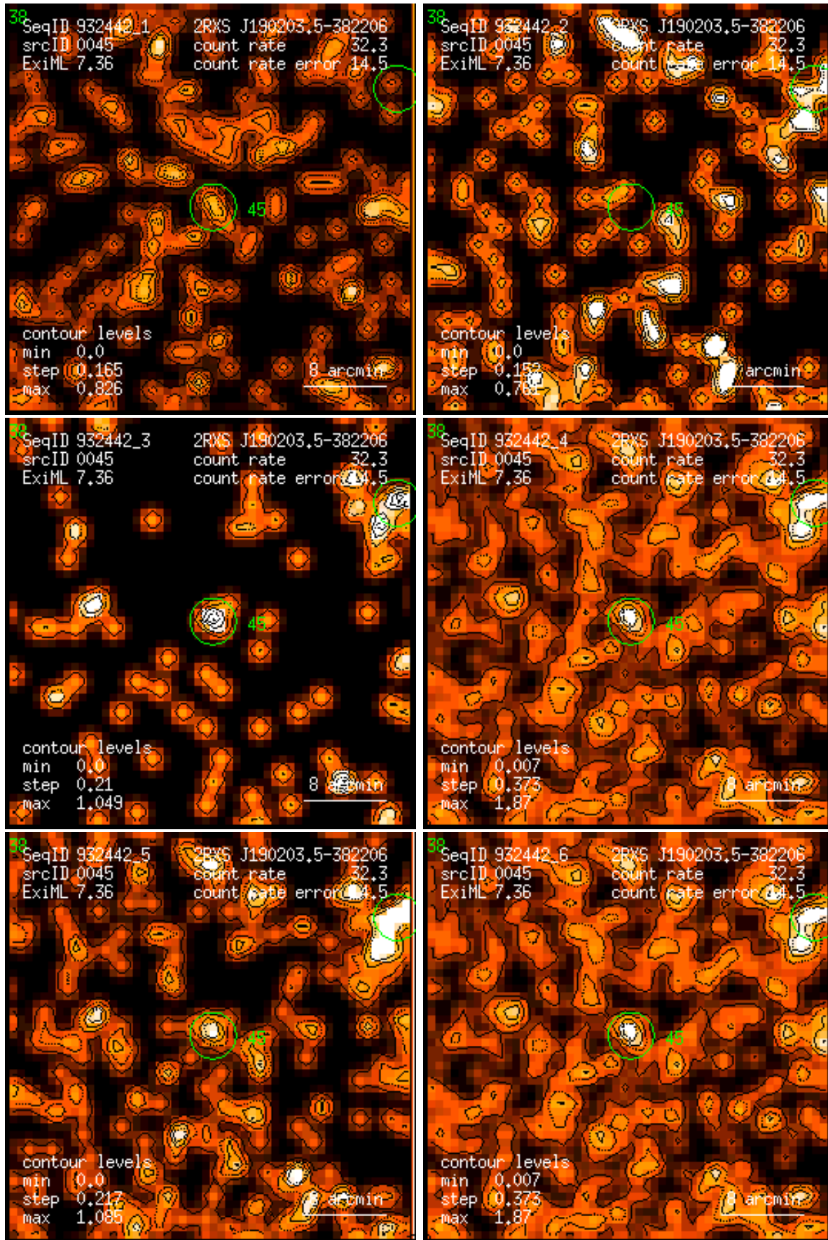
Figure 45: RASS 932442: detection 0045: band rate images, Gaussian filter: (1) PSPC channels 11 – 41, (2) 52 – 90, (3) 91 – 201, (4) 11 – 235, (5) 52 – 201, (6) 11 – 201. Broad band rates in counts/ks. Band rate contour levels in counts/ks/arcmin 2 .
