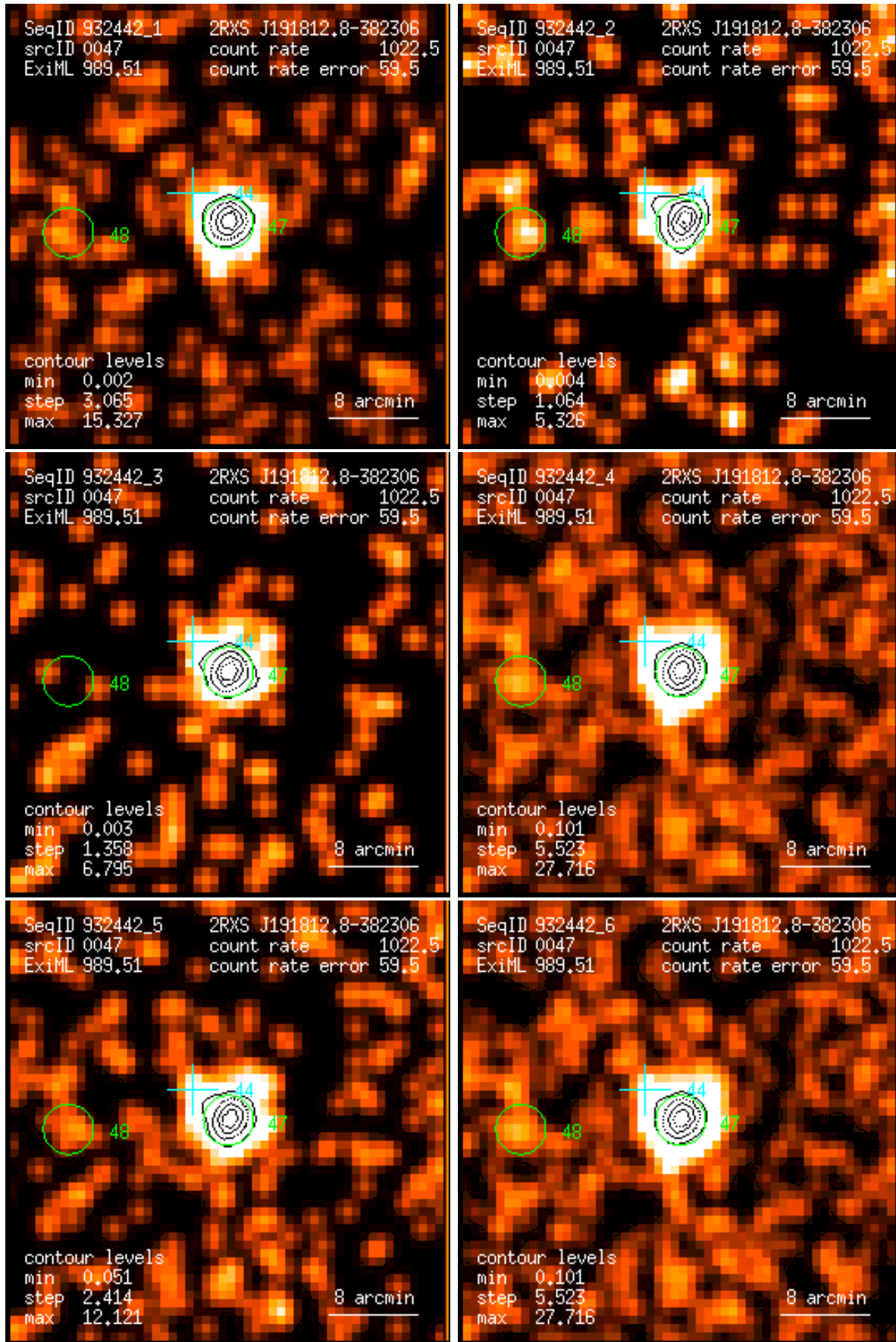
Figure 47: RASS 932442: detection 0047: band rate images, Gaussian filter: (1) PSPC channels 11 – 41, (2) 52 – 90, (3) 91 – 201, (4) 11 – 235, (5) 52 – 201, (6) 11 – 201. Broad band rates in counts/ks. Band rate contour levels in counts/ks/arcmin 2 .
