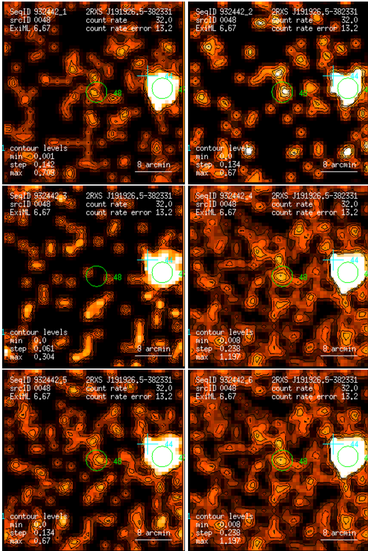
Figure 48: RASS 932442: detection 0048: band rate images, Gaussian filter: (1) PSPC channels 11 – 41, (2) 52 – 90, (3) 91 – 201, (4) 11 – 235, (5) 52 – 201, (6) 11 – 201. Broad band rates in counts/ks. Band rate contour levels in counts/ks/arcmin 2 .
