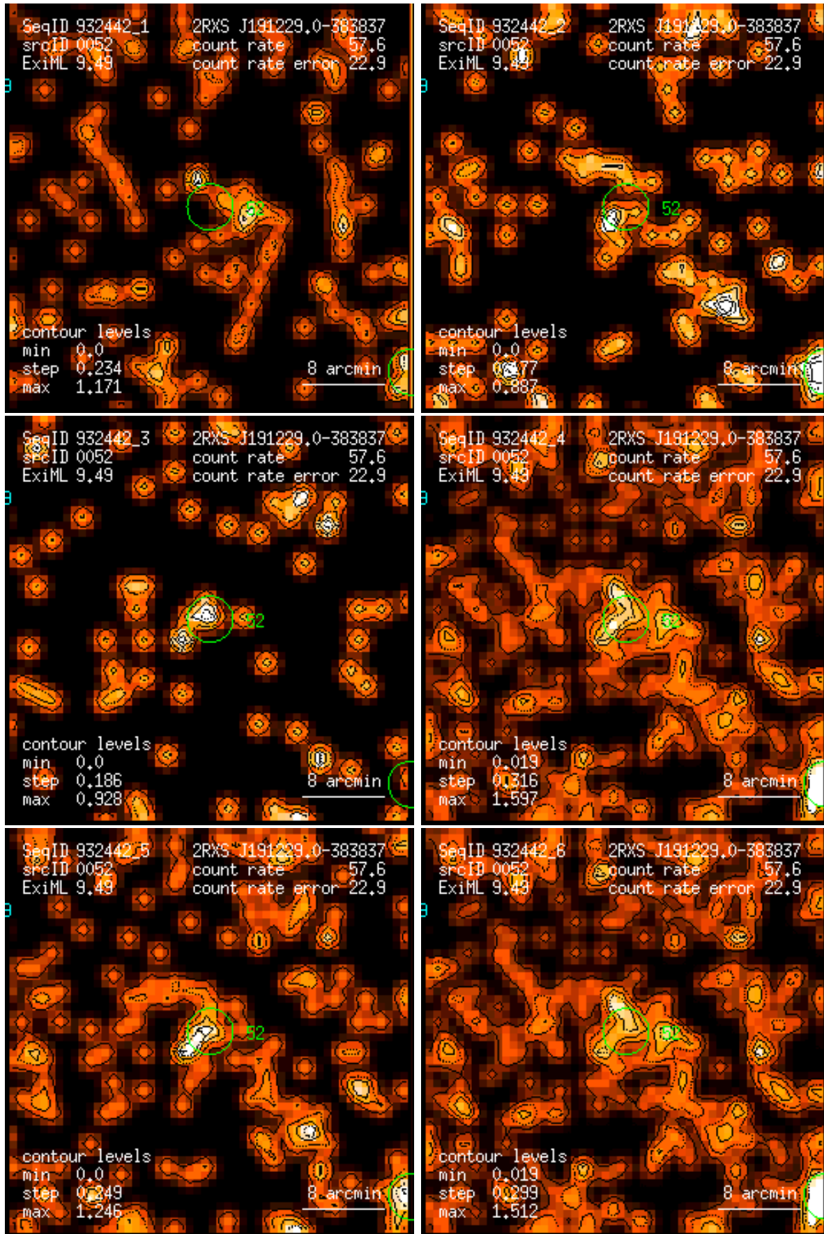
Figure 52: RASS 932442: detection 0052: band rate images, Gaussian filter: (1) PSPC channels 11 – 41, (2) 52 – 90, (3) 91 – 201, (4) 11 – 235, (5) 52 – 201, (6) 11 – 201. Broad band rates in counts/ks. Band rate contour levels in counts/ks/arcmin 2 .
