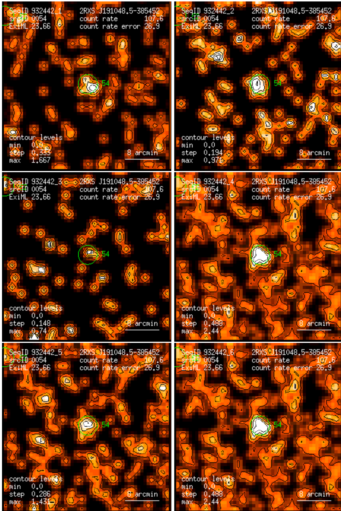
Figure 54: RASS 932442: detection 0054: band rate images, Gaussian filter: (1) PSPC channels 11 – 41, (2) 52 – 90, (3) 91 – 201, (4) 11 – 235, (5) 52 – 201, (6) 11 – 201. Broad band rates in counts/ks. Band rate contour levels in counts/ks/arcmin 2 .
