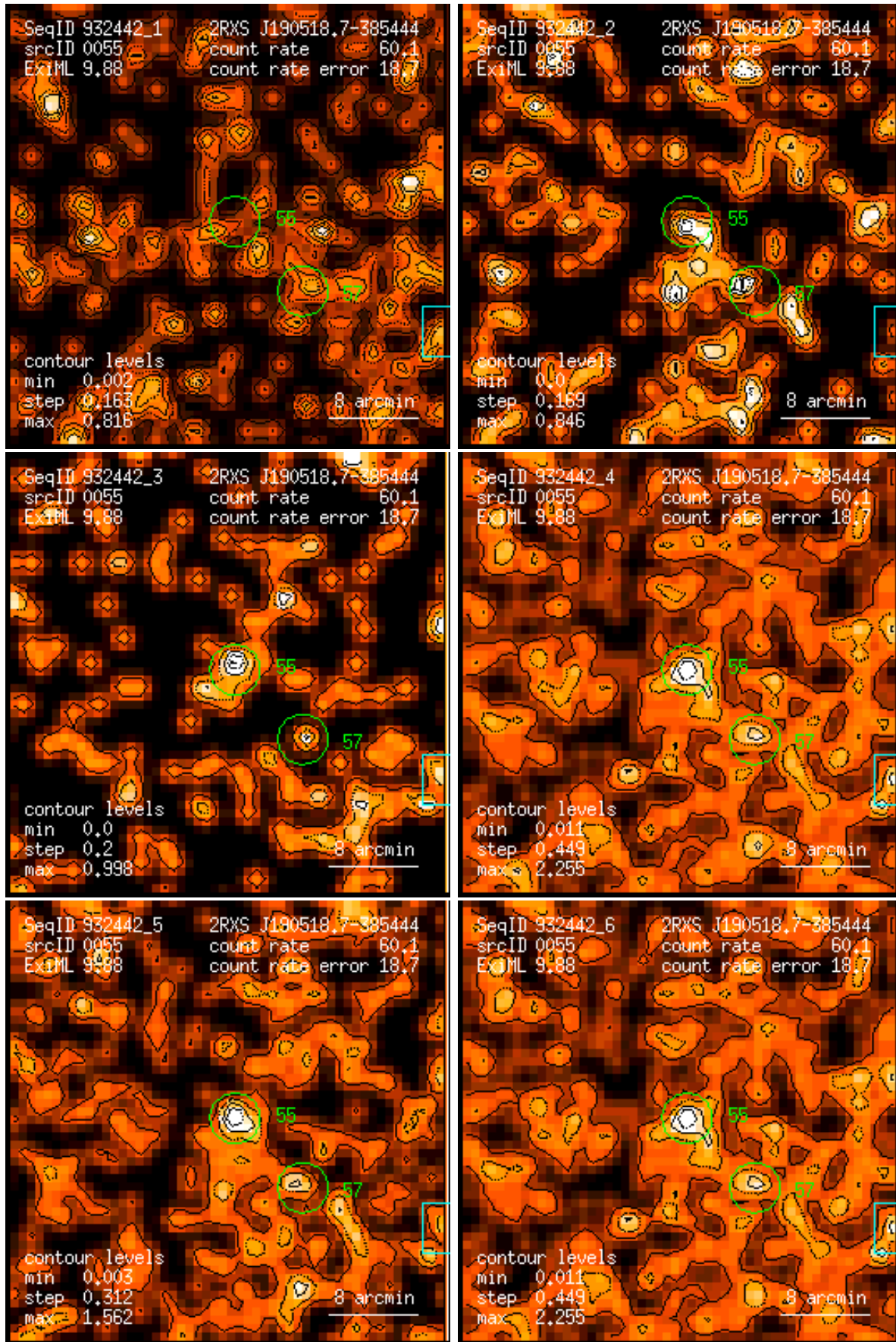
Figure 55: RASS 932442: detection 0055: band rate images, Gaussian filter: (1) PSPC channels 11 – 41, (2) 52 – 90, (3) 91 – 201, (4) 11 – 235, (5) 52 – 201, (6) 11 – 201. Broad band rates in counts/ks. Band rate contour levels in counts/ks/arcmin 2 .
