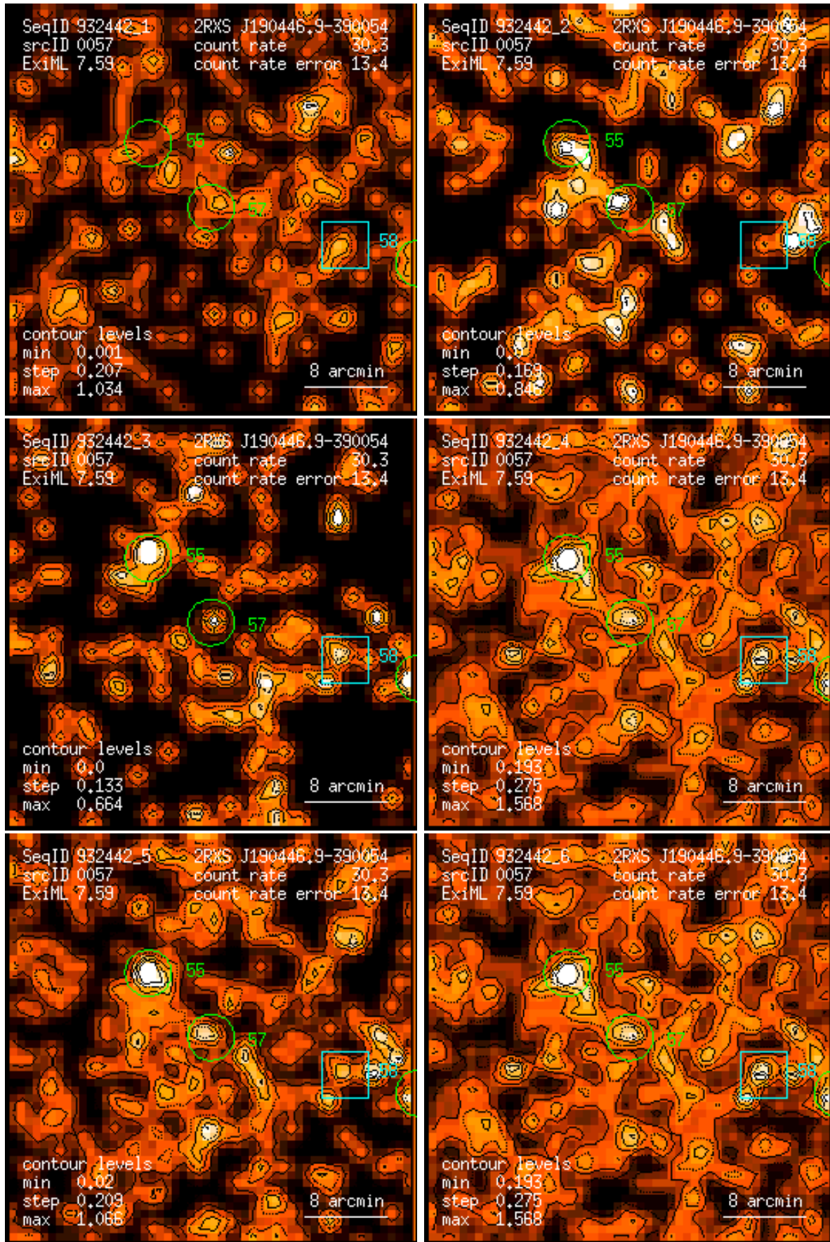
Figure 57: RASS 932442: detection 0057: band rate images, Gaussian filter: (1) PSPC channels 11 – 41, (2) 52 – 90, (3) 91 – 201, (4) 11 – 235, (5) 52 – 201, (6) 11 – 201. Broad band rates in counts/ks. Band rate contour levels in counts/ks/arcmin 2 .
