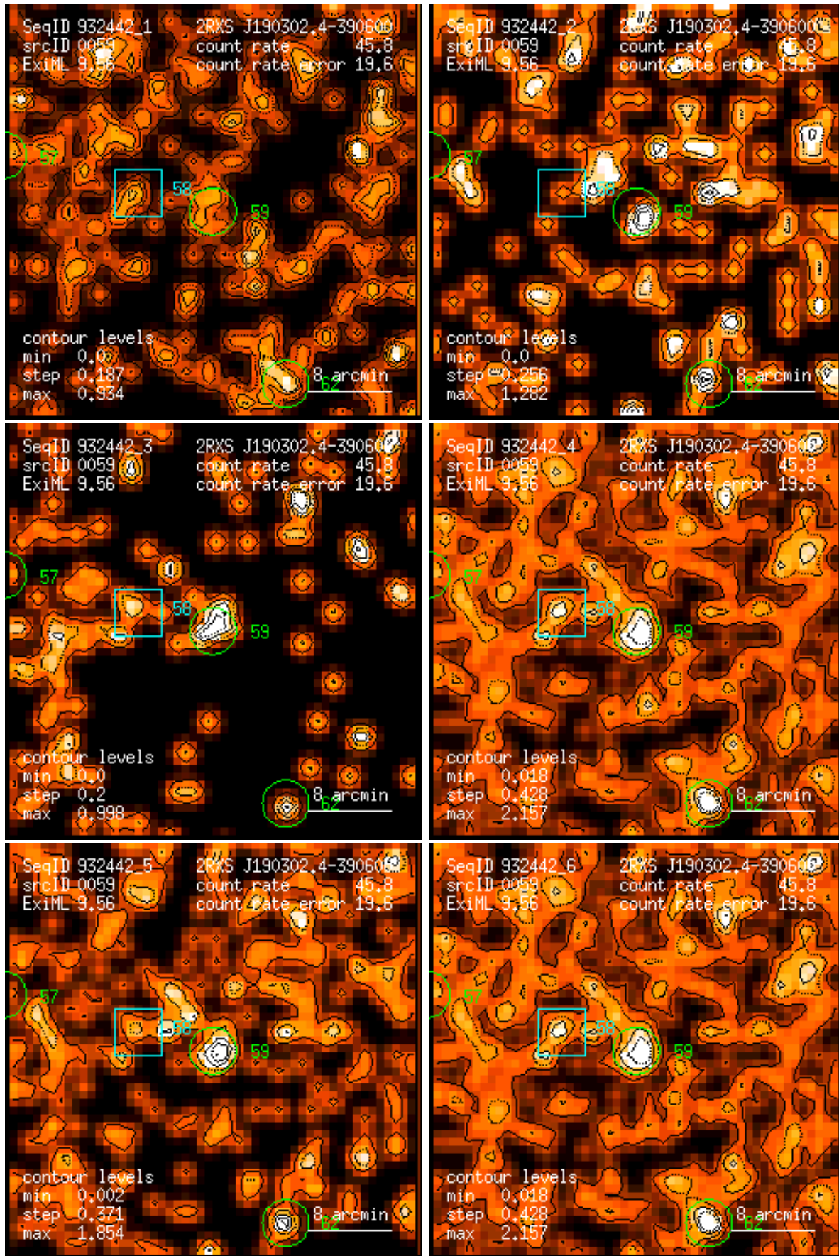
Figure 59: RASS 932442: detection 0059: band rate images, Gaussian filter: (1) PSPC channels 11 – 41, (2) 52 – 90, (3) 91 – 201, (4) 11 – 235, (5) 52 – 201, (6) 11 – 201. Broad band rates in counts/ks. Band rate contour levels in counts/ks/arcmin 2 .
