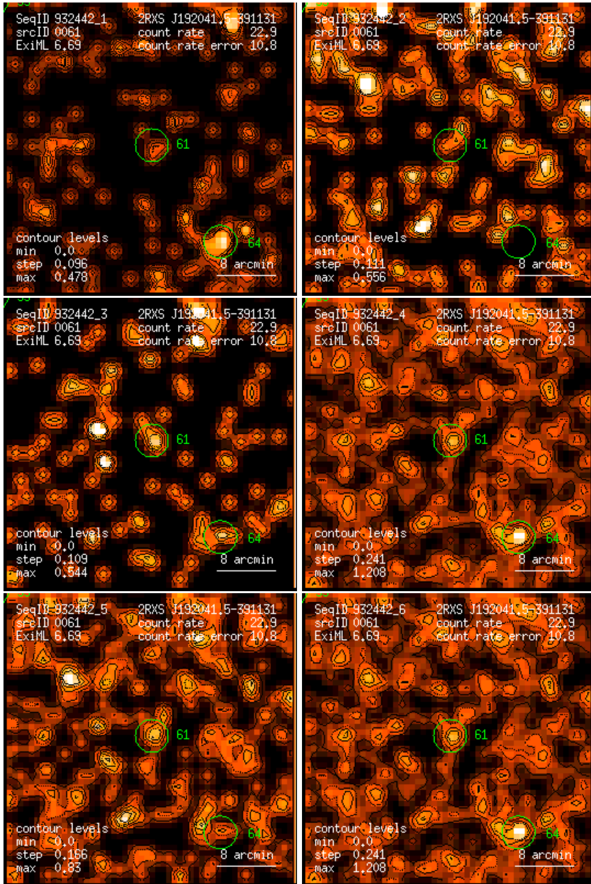
Figure 61: RASS 932442: detection 0061: band rate images, Gaussian filter: (1) PSPC channels 11 – 41, (2) 52 – 90, (3) 91 – 201, (4) 11 – 235, (5) 52 – 201, (6) 11 – 201. Broad band rates in counts/ks. Band rate contour levels in counts/ks/arcmin 2 .
