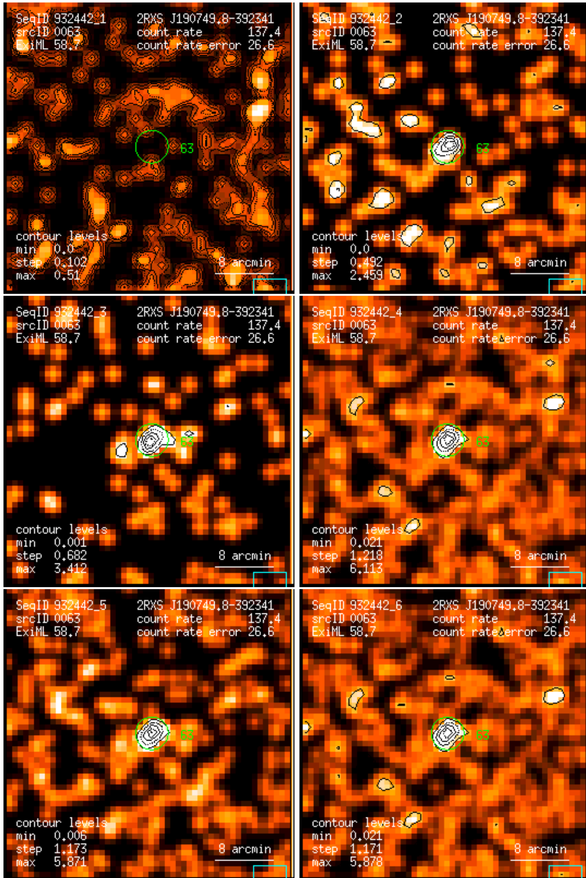
Figure 63: RASS 932442: detection 0063: band rate images, Gaussian filter: (1) PSPC channels 11 – 41, (2) 52 – 90, (3) 91 – 201, (4) 11 – 235, (5) 52 – 201, (6) 11 – 201. Broad band rates in counts/ks. Band rate contour levels in counts/ks/arcmin 2 .
