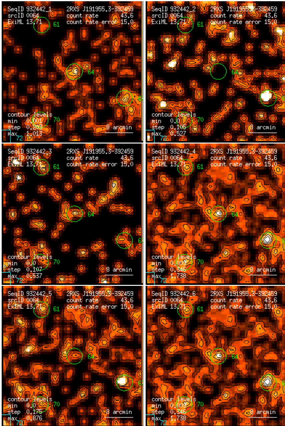
Figure 64: RASS 932442: detection 0064: band rate images, Gaussian filter: (1) PSPC channels 11 – 41, (2) 52 – 90, (3) 91 – 201, (4) 11 – 235, (5) 52 – 201, (6) 11 – 201. Broad band rates in counts/ks. Band rate contour levels in counts/ks/arcmin 2 .
