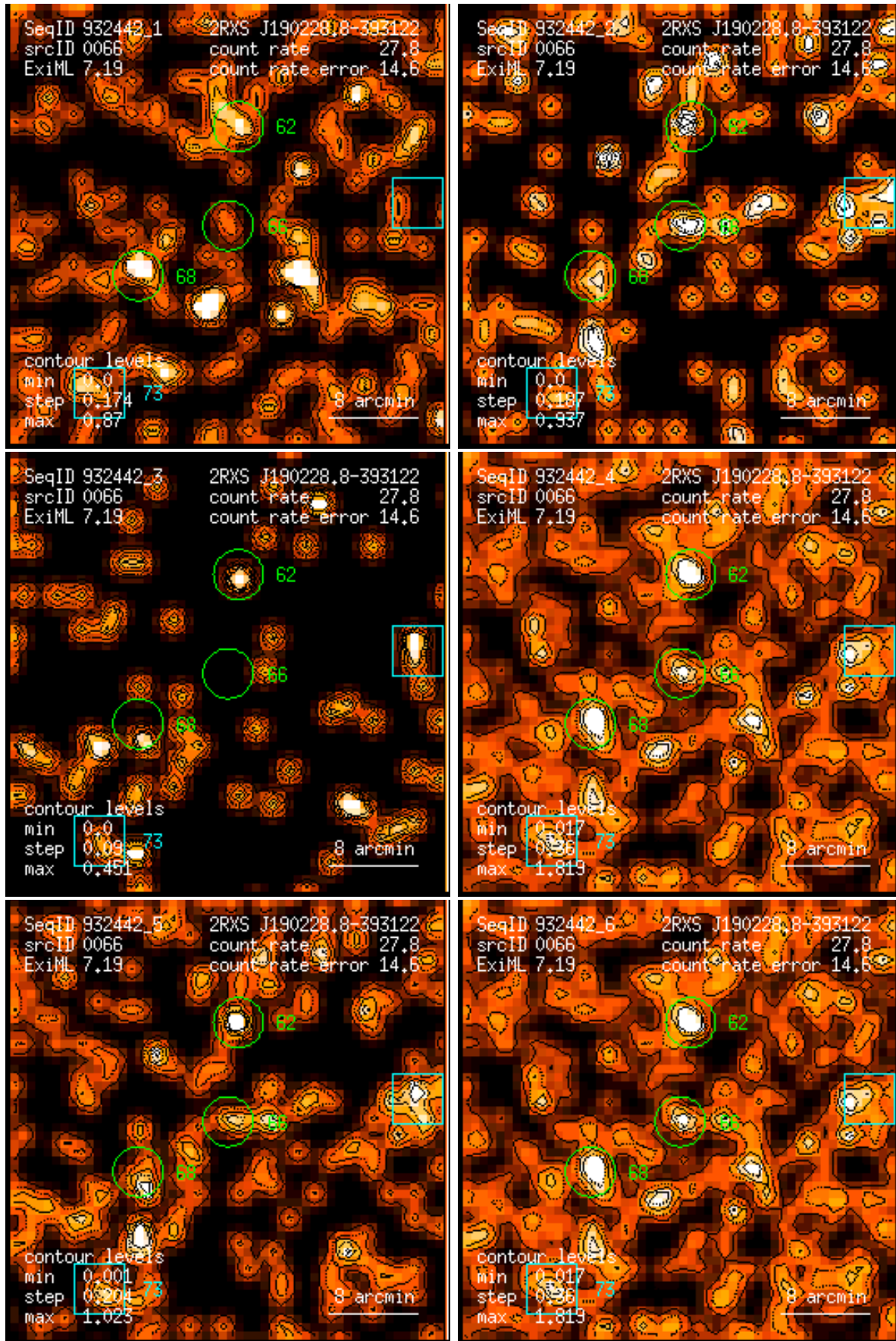
Figure 66: RASS 932442: detection 0066: band rate images, Gaussian filter: (1) PSPC channels 11 – 41, (2) 52 – 90, (3) 91 – 201, (4) 11 – 235, (5) 52 – 201, (6) 11 – 201. Broad band rates in counts/ks. Band rate contour levels in counts/ks/arcmin 2 .
