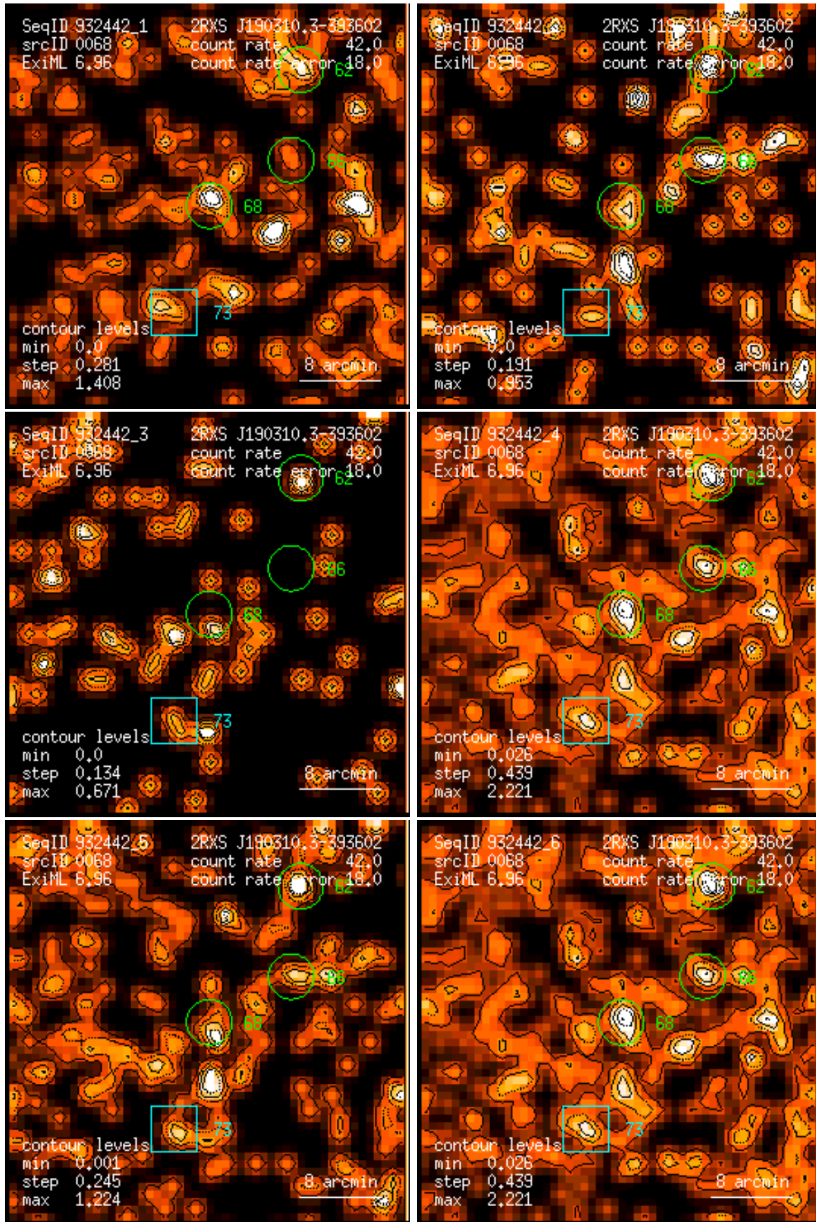
Figure 68: RASS 932442: detection 0068: band rate images, Gaussian filter: (1) PSPC channels 11 – 41, (2) 52 – 90, (3) 91 – 201, (4) 11 – 235, (5) 52 – 201, (6) 11 – 201. Broad band rates in counts/ks. Band rate contour levels in counts/ks/arcmin 2 .
