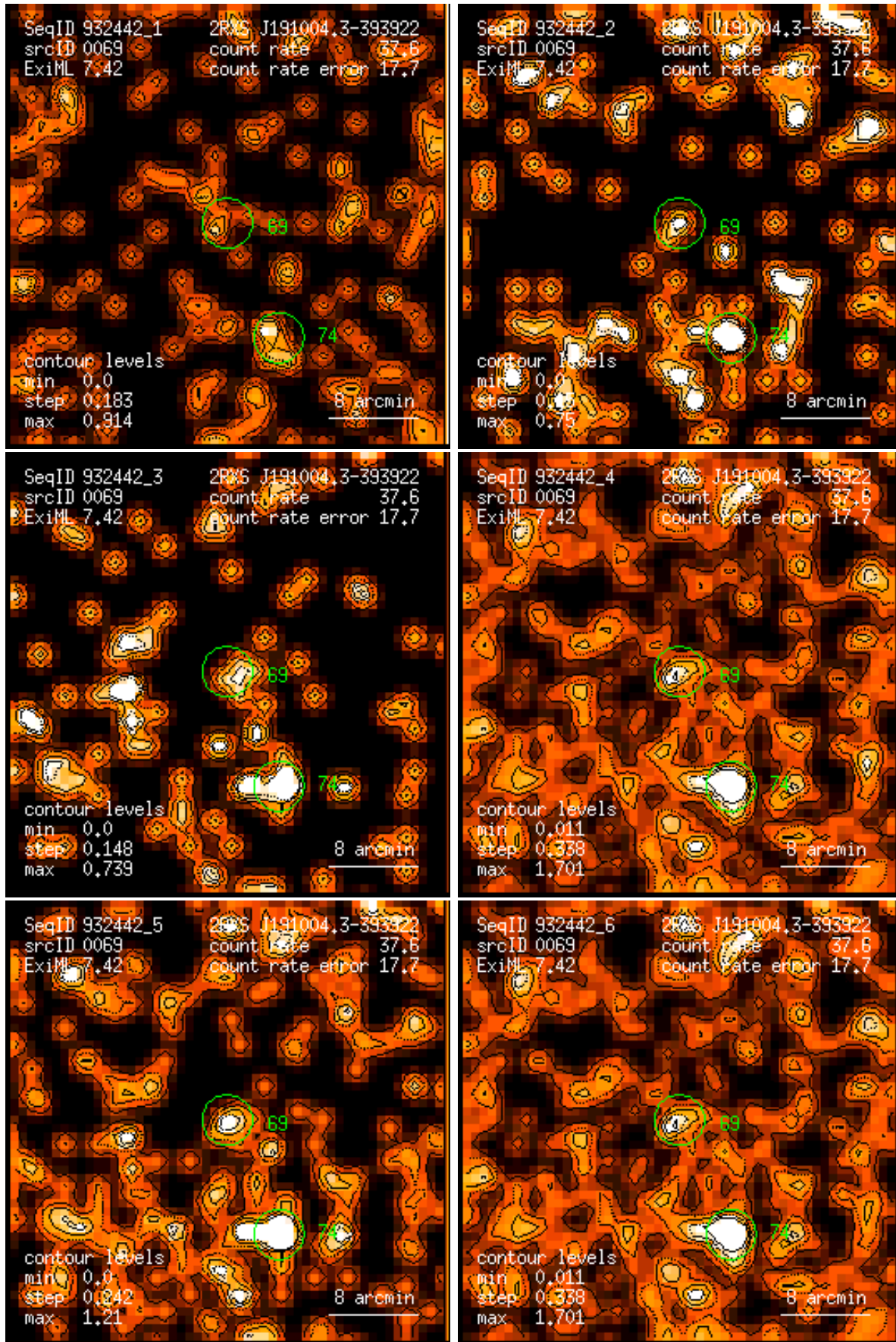
Figure 69: RASS 932442: detection 0069: band rate images, Gaussian filter: (1) PSPC channels 11 – 41, (2) 52 – 90, (3) 91 – 201, (4) 11 – 235, (5) 52 – 201, (6) 11 – 201. Broad band rates in counts/ks. Band rate contour levels in counts/ks/arcmin 2 .
