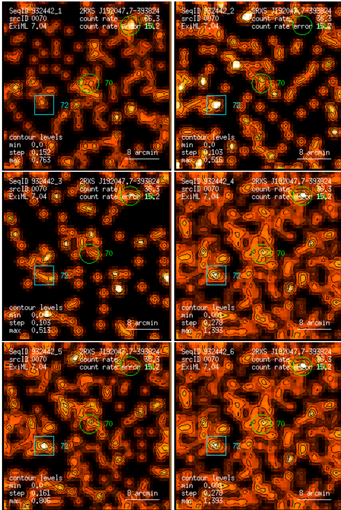
Figure 70: RASS 932442: detection 0070: band rate images, Gaussian filter: (1) PSPC channels 11 – 41, (2) 52 – 90, (3) 91 – 201, (4) 11 – 235, (5) 52 – 201, (6) 11 – 201. Broad band rates in counts/ks. Band rate contour levels in counts/ks/arcmin 2 .
