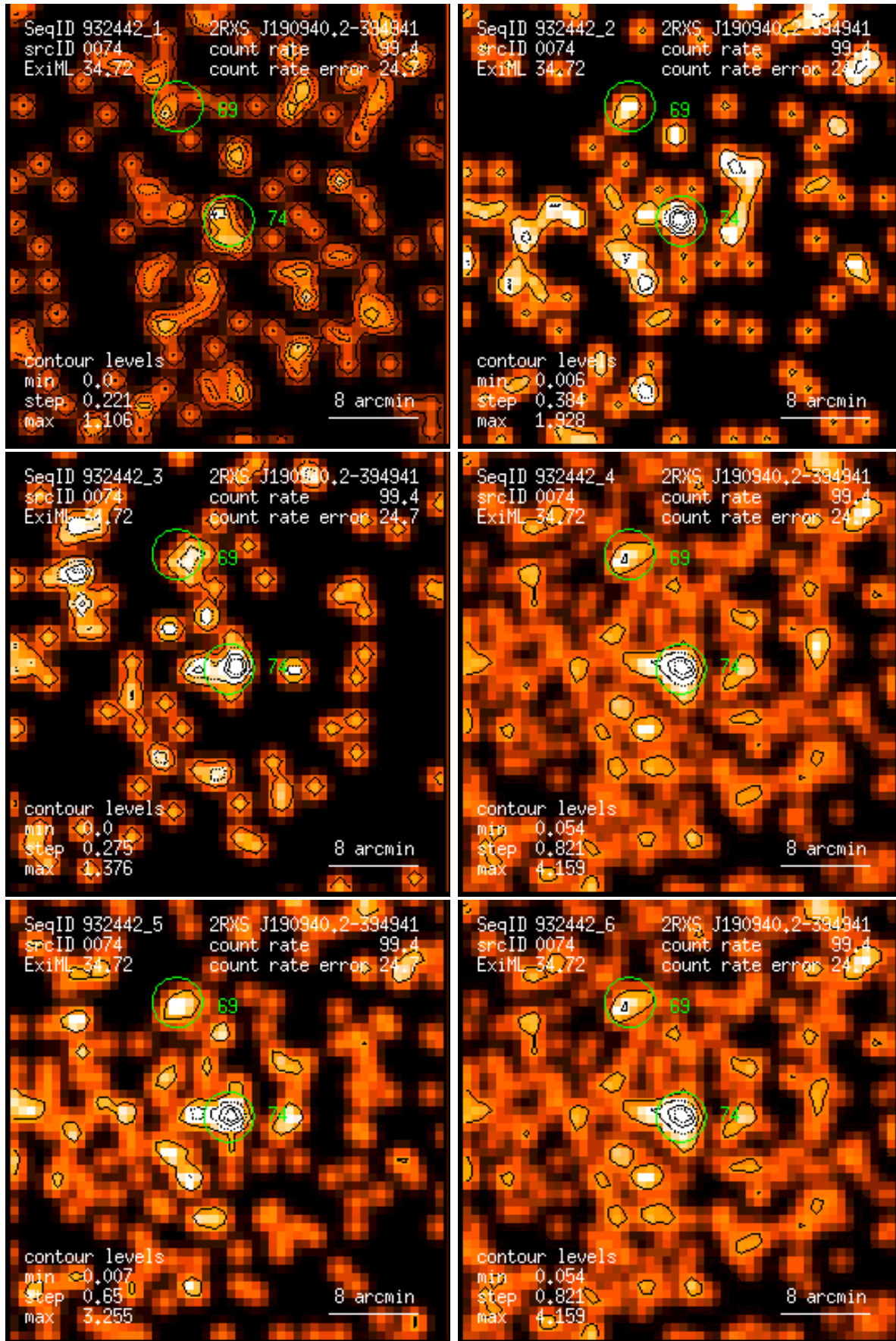
Figure 74: RASS 932442: detection 0074: band rate images, Gaussian filter: (1) PSPC channels 11 – 41, (2) 52 – 90, (3) 91 – 201, (4) 11 – 235, (5) 52 – 201, (6) 11 – 201. Broad band rates in counts/ks. Band rate contour levels in counts/ks/arcmin 2 .
