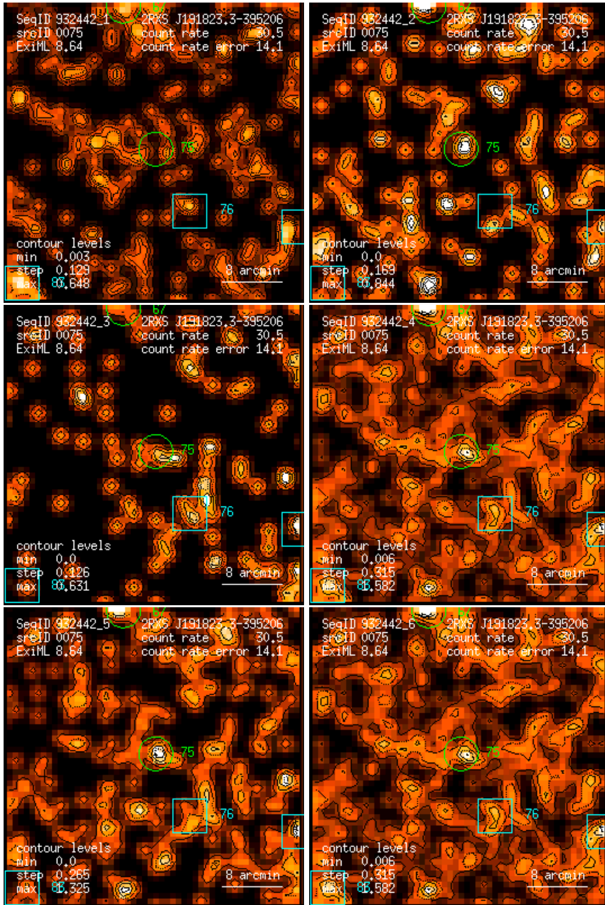
Figure 75: RASS 932442: detection 0075: band rate images, Gaussian filter: (1) PSPC channels 11 – 41, (2) 52 – 90, (3) 91 – 201, (4) 11 – 235, (5) 52 – 201, (6) 11 – 201. Broad band rates in counts/ks. Band rate contour levels in counts/ks/arcmin 2 .
