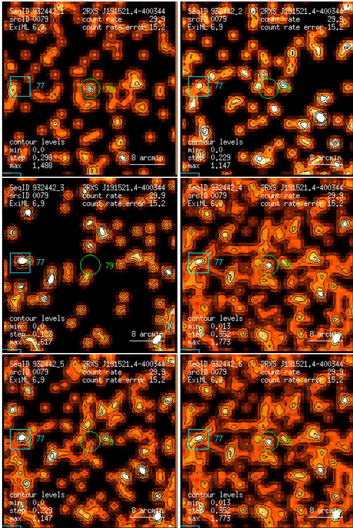
Figure 79: RASS 932442: detection 0079: band rate images, Gaussian filter: (1) PSPC channels 11 – 41, (2) 52 – 90, (3) 91 – 201, (4) 11 – 235, (5) 52 – 201, (6) 11 – 201. Broad band rates in counts/ks. Band rate contour levels in counts/ks/arcmin 2 .
