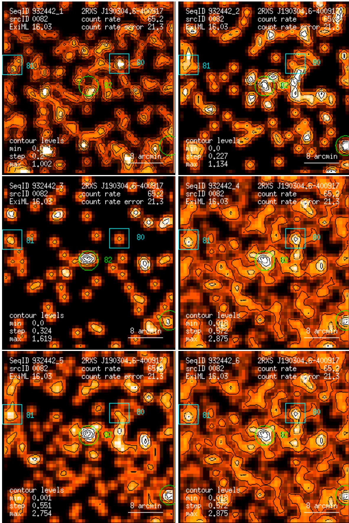
Figure 82: RASS 932442: detection 0082: band rate images, Gaussian filter: (1) PSPC channels 11 – 41, (2) 52 – 90, (3) 91 – 201, (4) 11 – 235, (5) 52 – 201, (6) 11 – 201. Broad band rates in counts/ks. Band rate contour levels in counts/ks/arcmin 2 .
